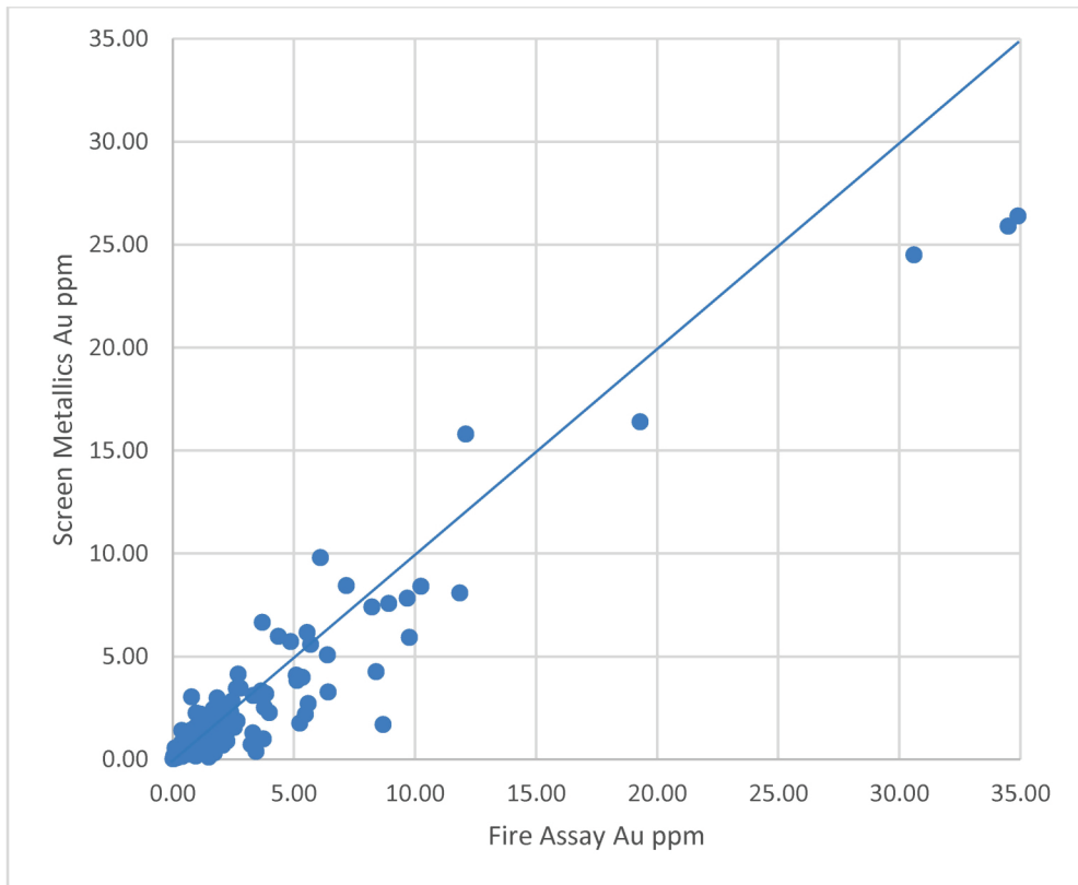
FIGURE 1 ALL 216 SCREEN METALLICS ASSAYS VS FIRE ASSAYS
