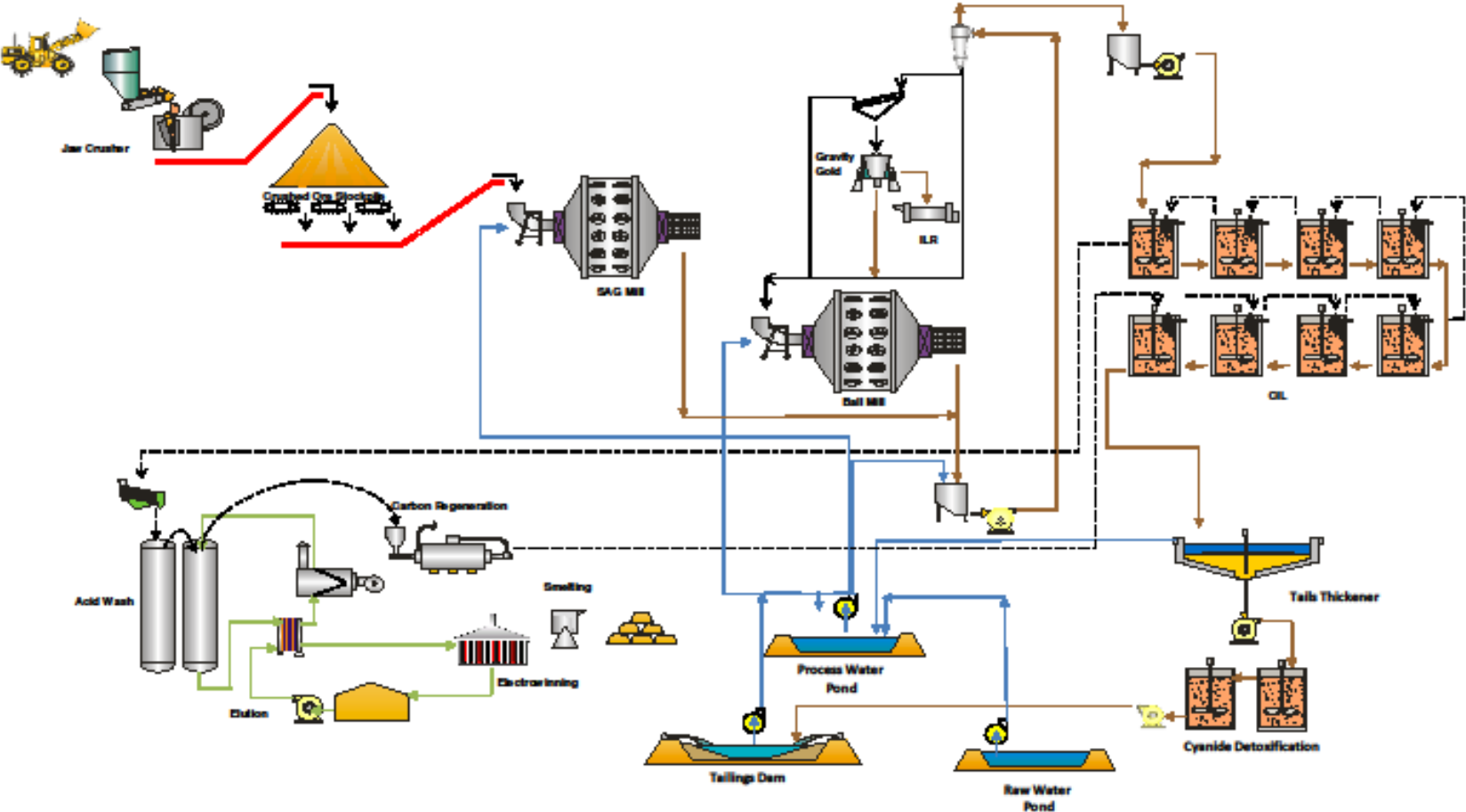
5272 Medusa Tambis: Draft Process Schematic
