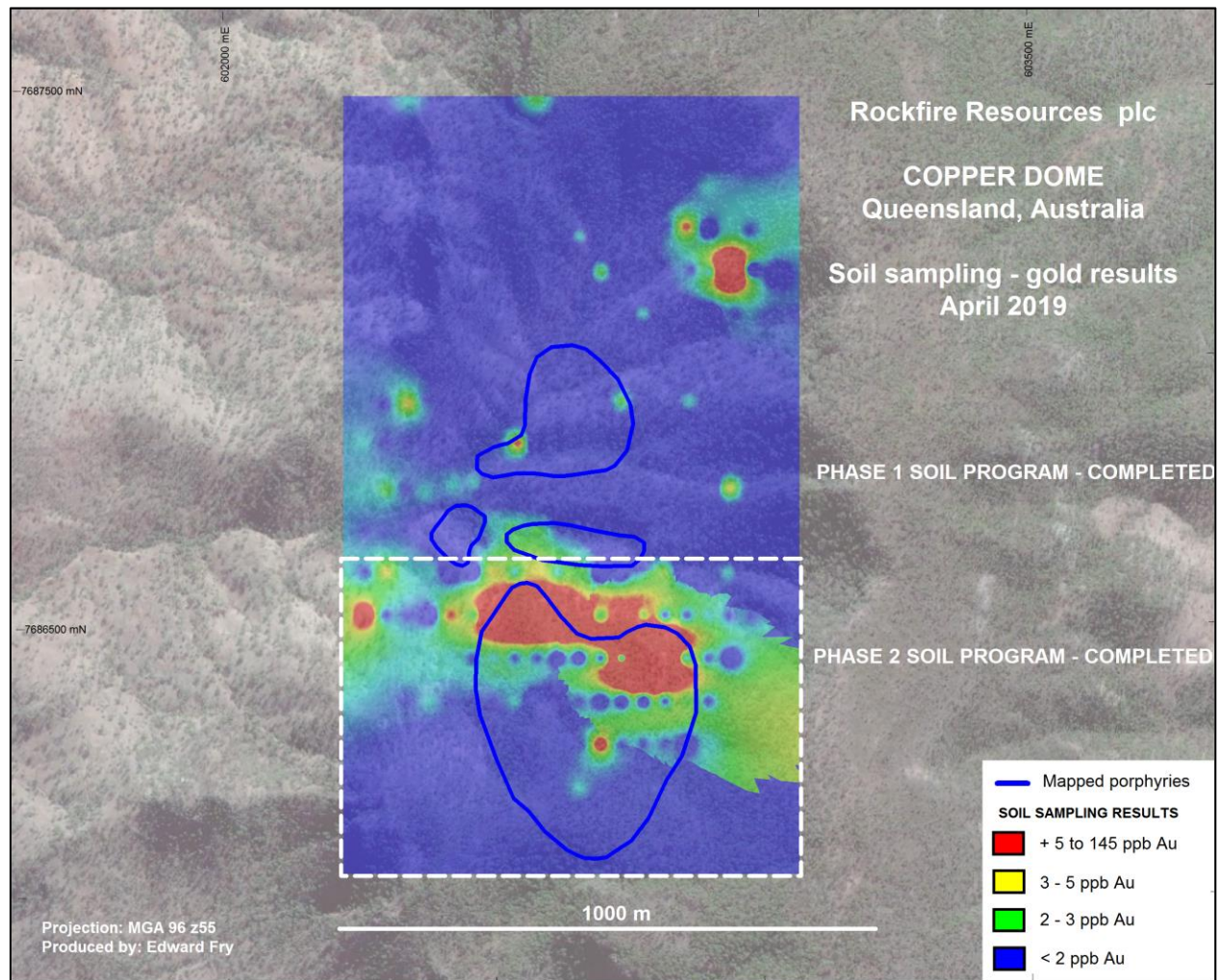
Gold-in-soil results
