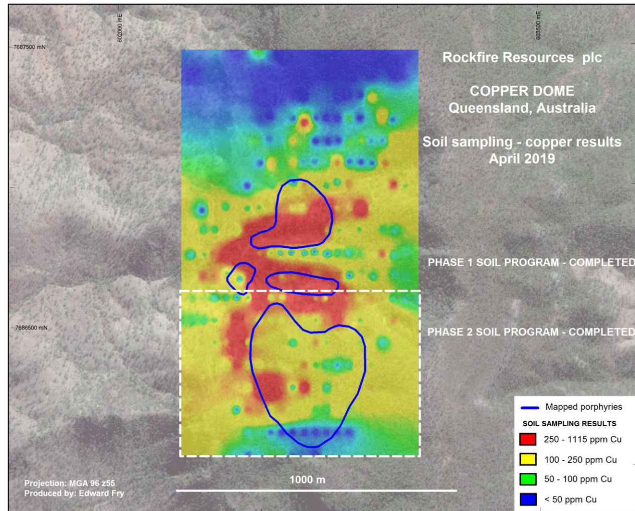
Copper-in-soil results
