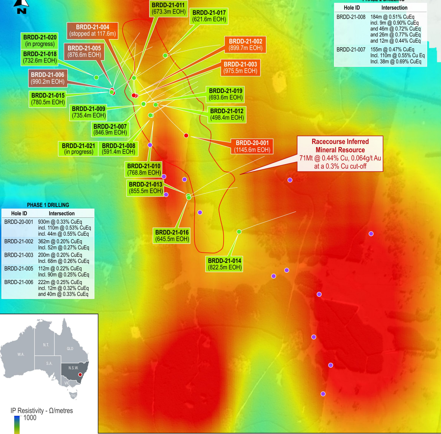
Image - IP Resistivity - depth slice 600m
