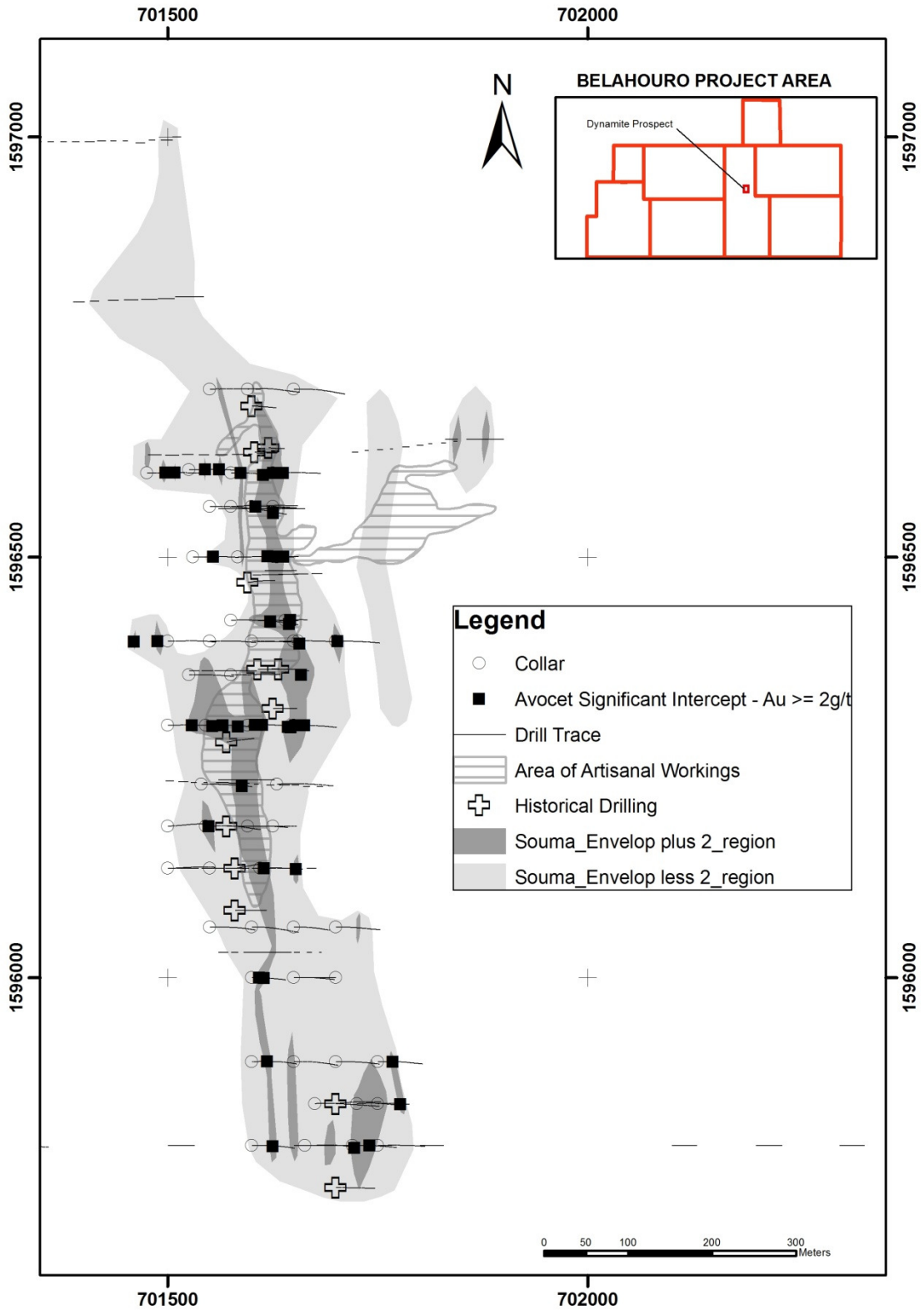
FIGURE 1 - DRILL HOLE PLAN FOR DYNAMITE, SOUMA TREND
