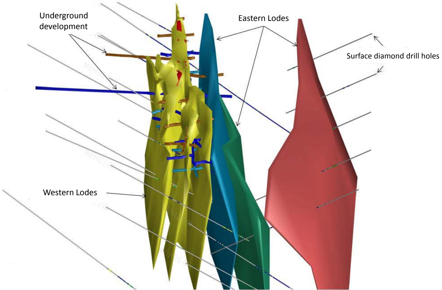
Figure 1: Mallappakonda Mine – 3D resource models and drilling, looking north
