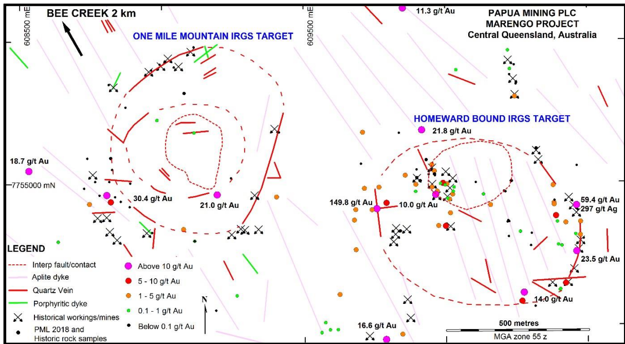
Structural interpretation map showing the One Mile Mountain and Homeward Bound targets and associated gold-in-rock results and historical workings at the Marengo Gold Project, Queensland, Australia
