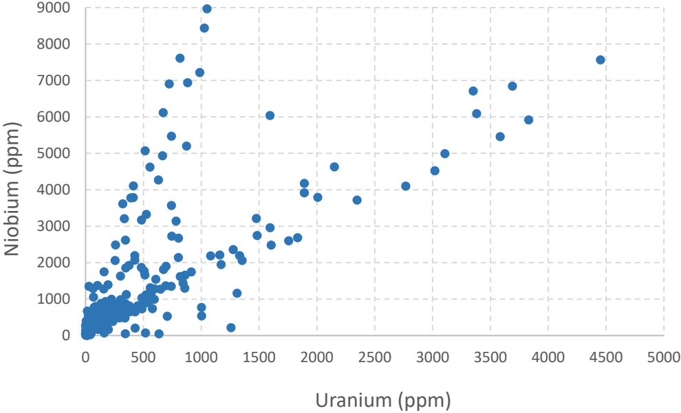
Scatterplot of U versus Nb
