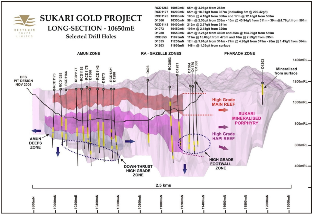
Figure 2 – Schematic Long section - 10650E; showing main target areas and recent high grade drilling results – Amun Deeps, Downthrust Zone and Pharaoh Zones
