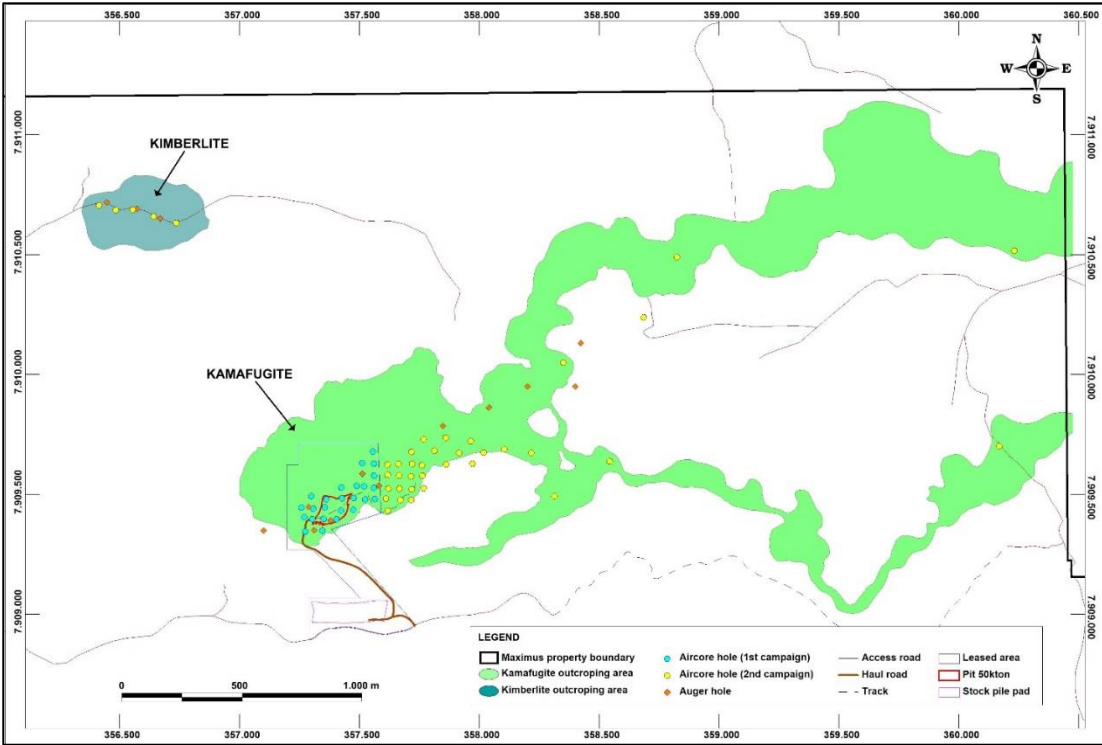
Figure 01 – Maximus Prospect - Air core drilling location
