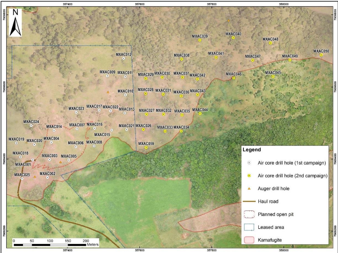
Figure 02 – Maximus Prospect - Air core holes distributed with grid spacing
