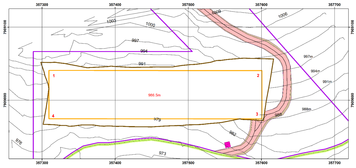
Figure 3: Plan of Stockpile Area
