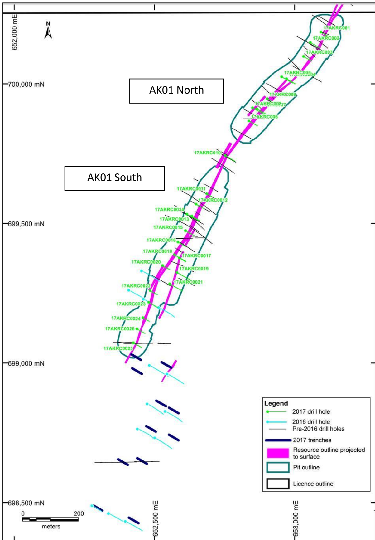
Figure 1. 2017 RC Pit Definition Drill Holes to the UTM (Universal Transverse Mercator) Co-ordinate System on the Akrokerri Licence
