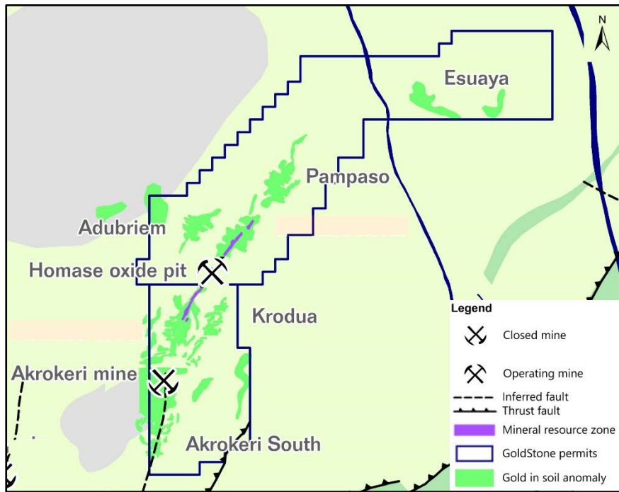
Figure 1: Plan of Geochemistry Soil Anomalies
