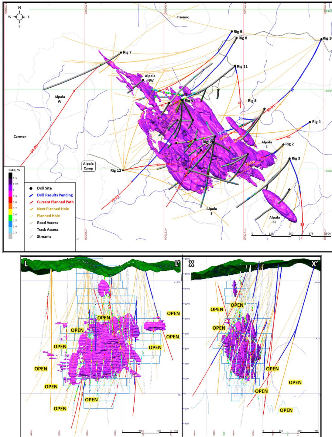
Figure 1: Drill hole location plan, showing copper-percent equivalent results to date and the traces of existing and planned drill holes. The Mineral Resource Estimate Grade shell at >1%CuEq is shown in magenta ( TOP ). NW-SE longitudinal-section ( BOTTOM LEFT ), and NE-SW cross-section ( BOTTOM RIGHT ) through the Alpa Deposit show Inferred block outlines (blue) and “open” areas marked for drill testing in the coming year. The results of the Mineral Resource Estimate released on 3 rd Jan 2018 are summarised below:
