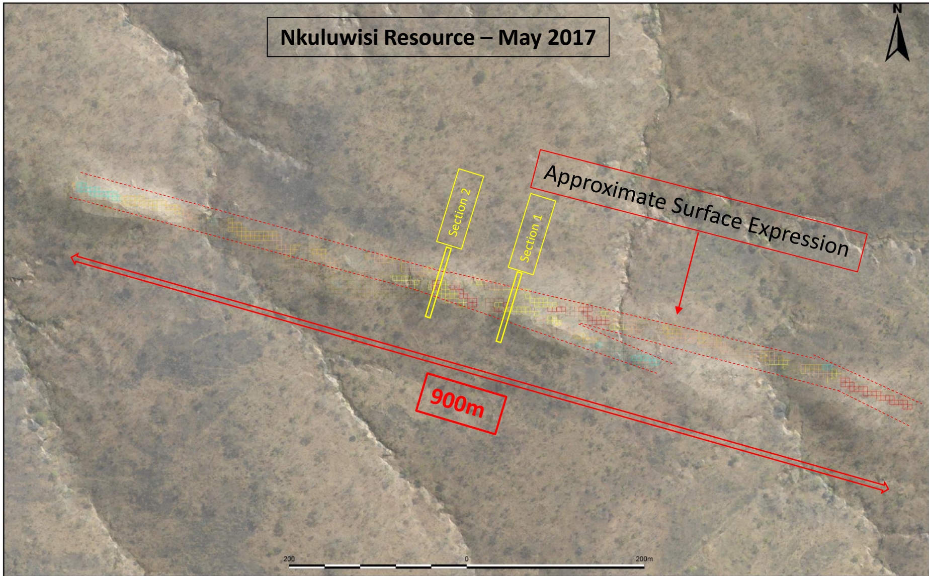
Figure 1: Orebody Surface Expression
