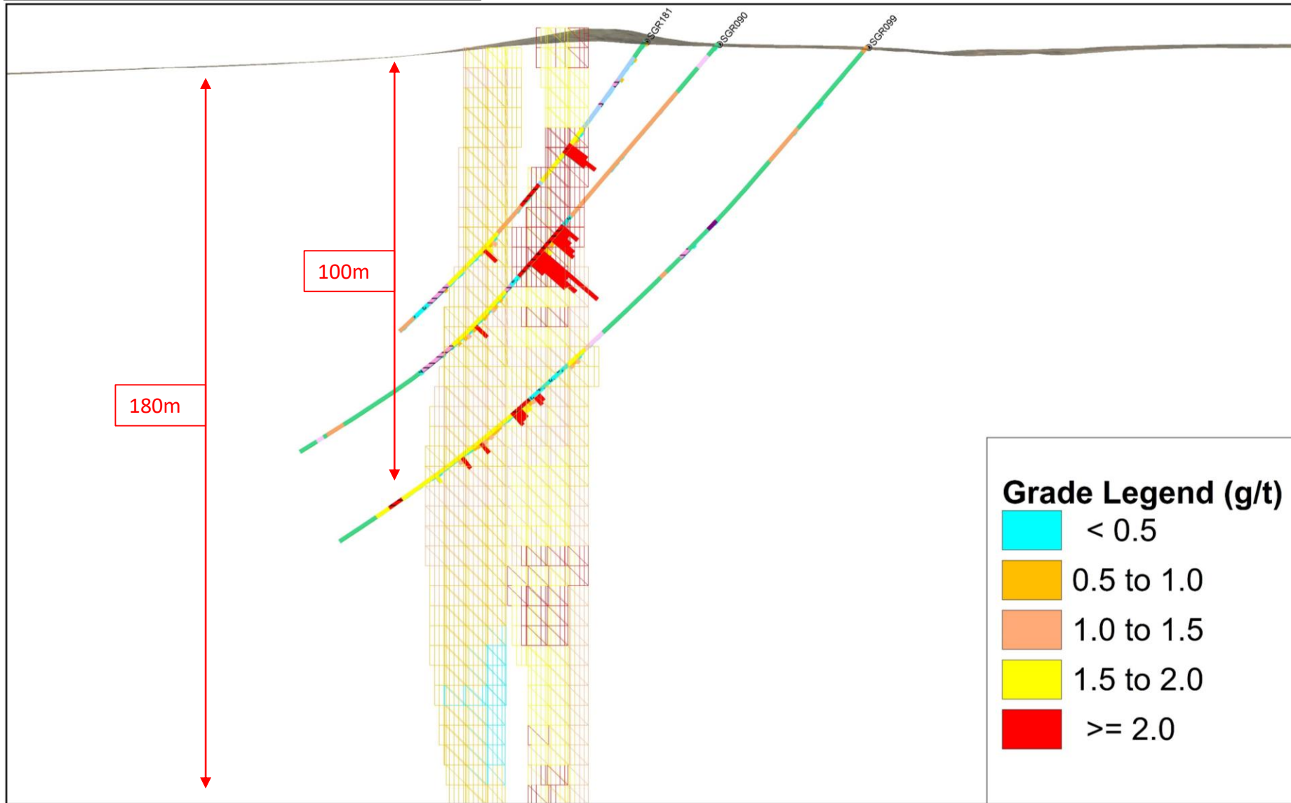
Figure 3: Section 1 Looking East
