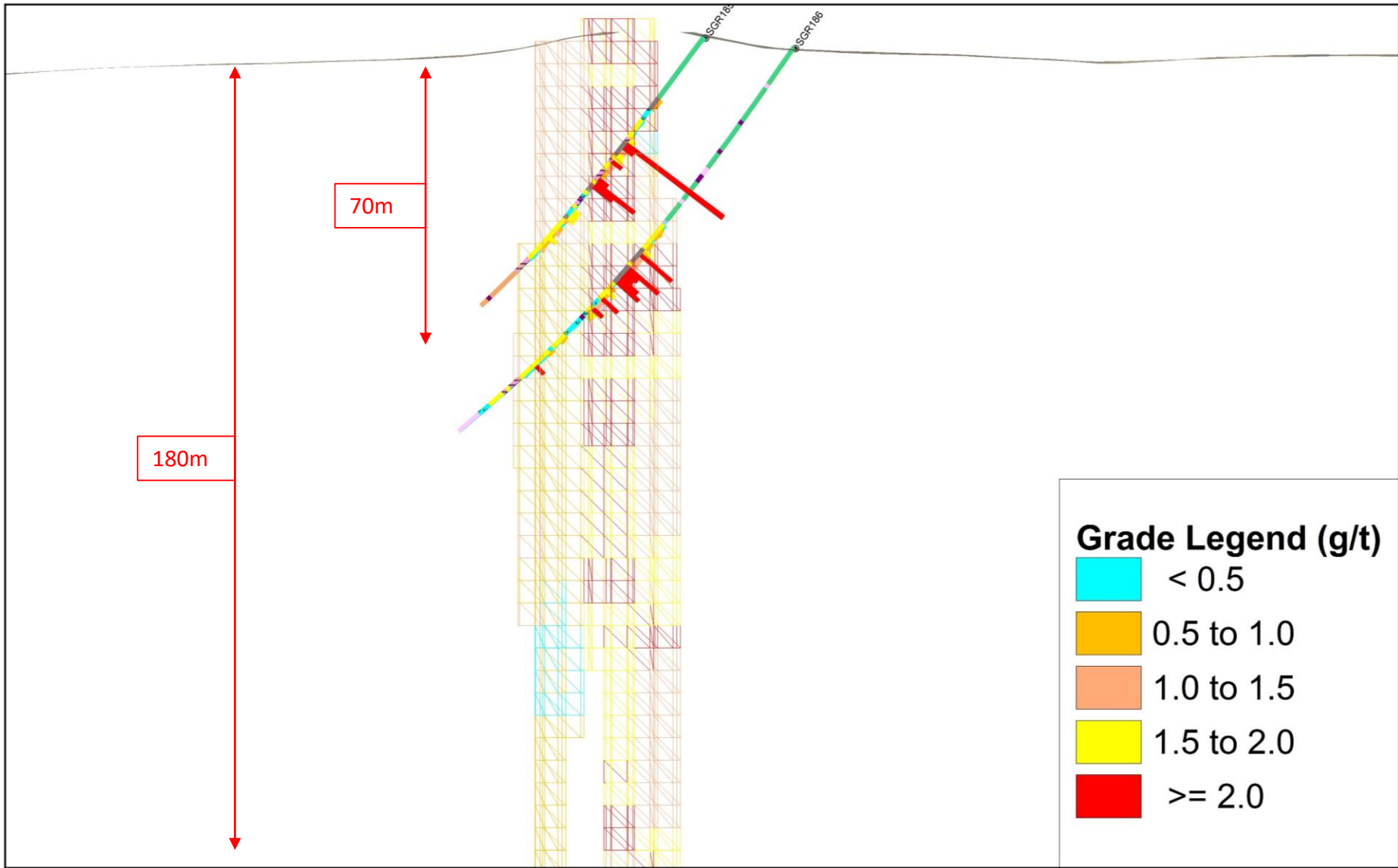
Figure 4: Section 2 Looking East
