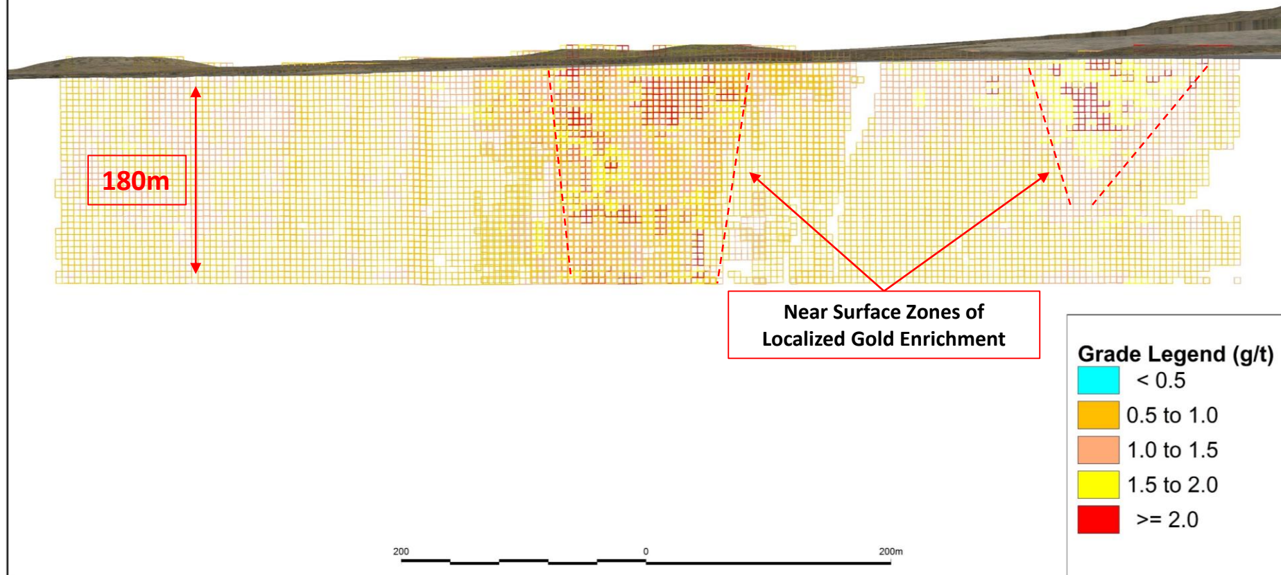
Figure 2: Longitudinal Section Looking North
