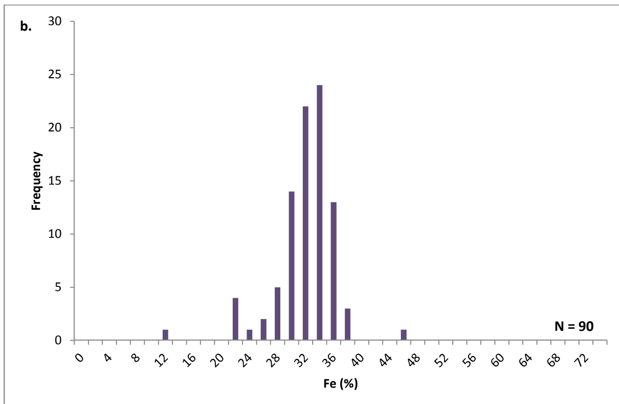
Figure 3: Histograms showing Fe distribution at a) Havik East and b) Havik Northeast
