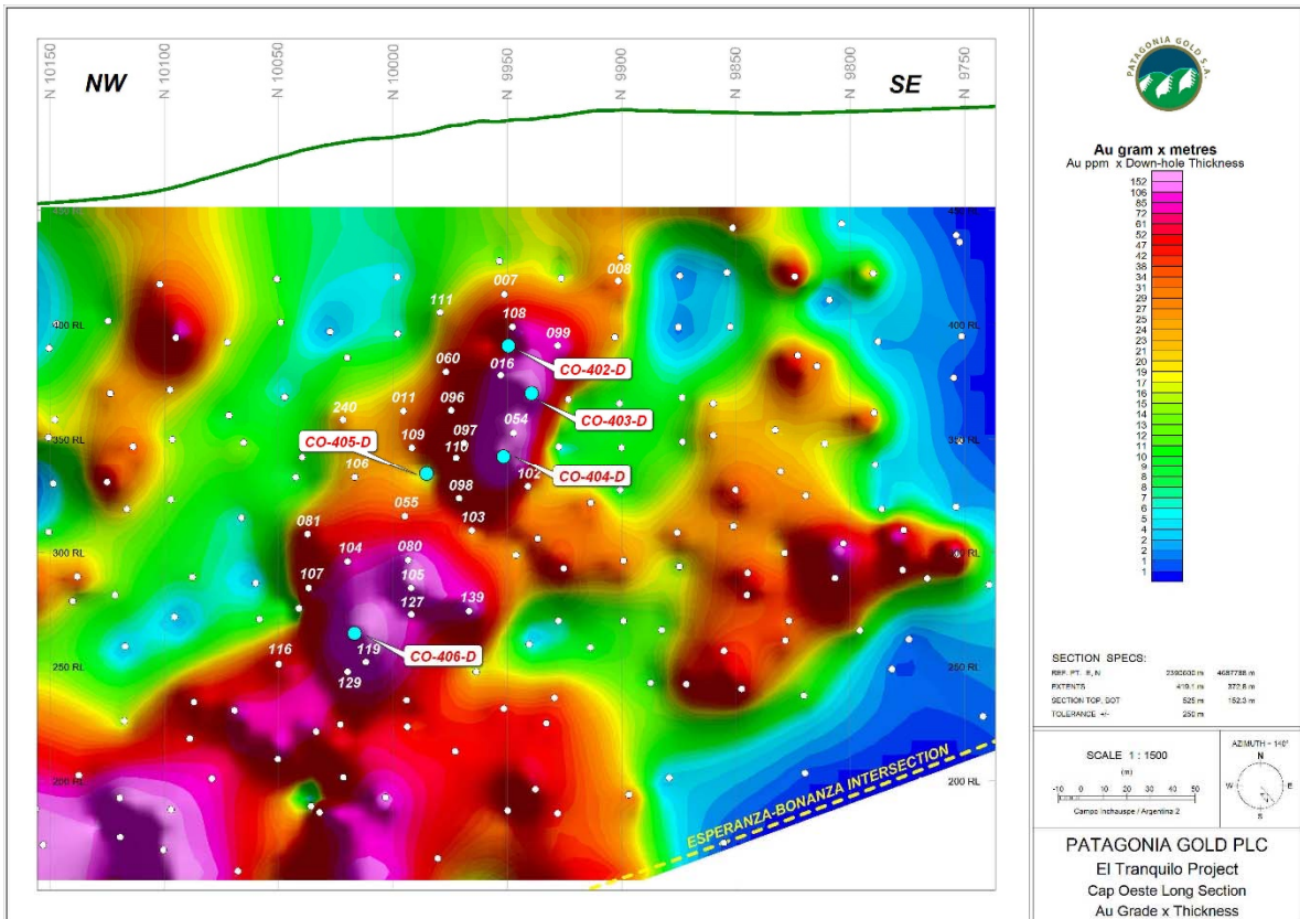
Figure 1; Cap-Oeste Long section of drill hole pierce points within high grade COSE Style shoot area with raster image of Au grade metres.
