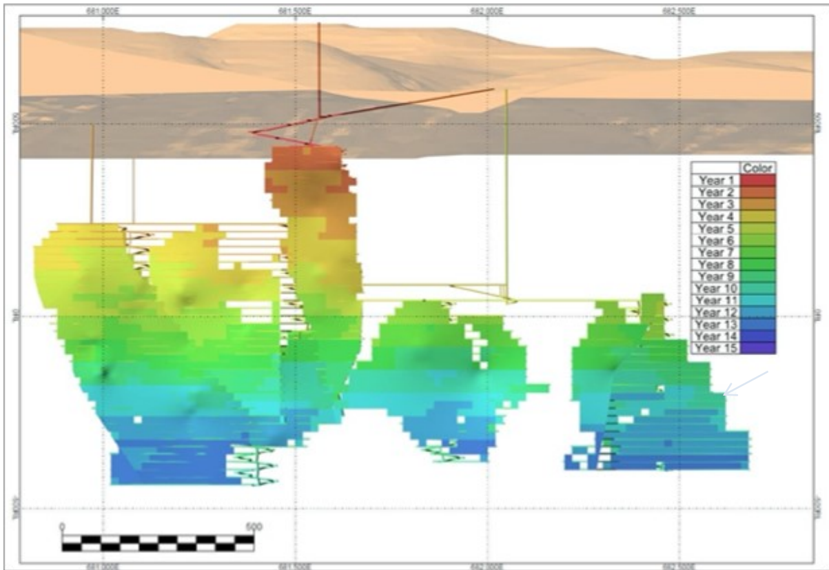
Figure 1: Toral Life of Mine Development Plan (looking North) with the current phase of the 2021 drilling campaign retrieving resource, geotechnical and metallurgical data to develop the early years of a potential future mining scenario.
