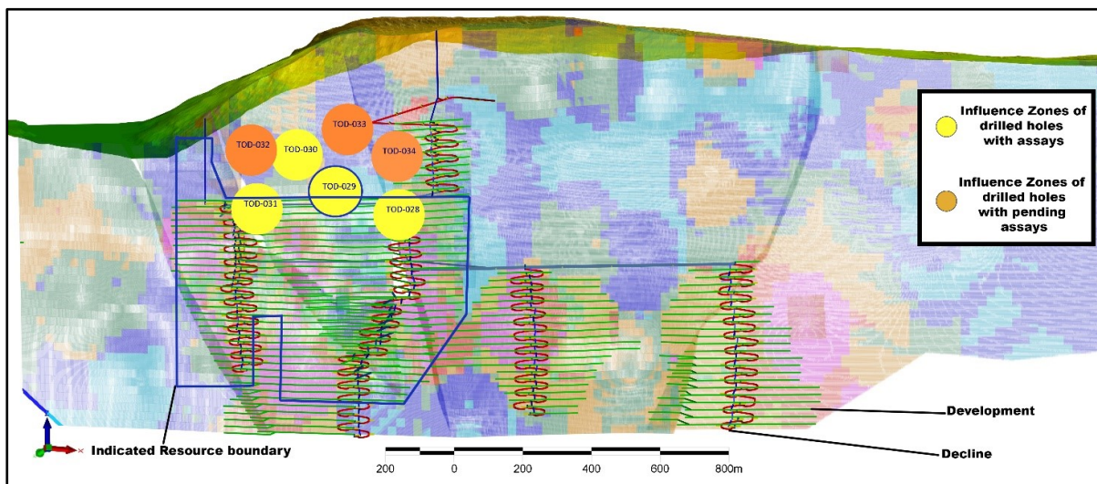
Figures 2 & 3: East-West long sections locating completed primary drill holes TOD-028, 029, 030 & 031 (2021 drilling campaign), the blue circle indicates area of TOD-029 and its daughter holes.
