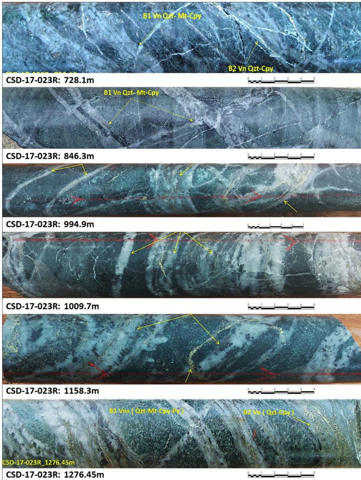
Figure 2: Selected examples of mineralisation encountered in Hole 23R.
