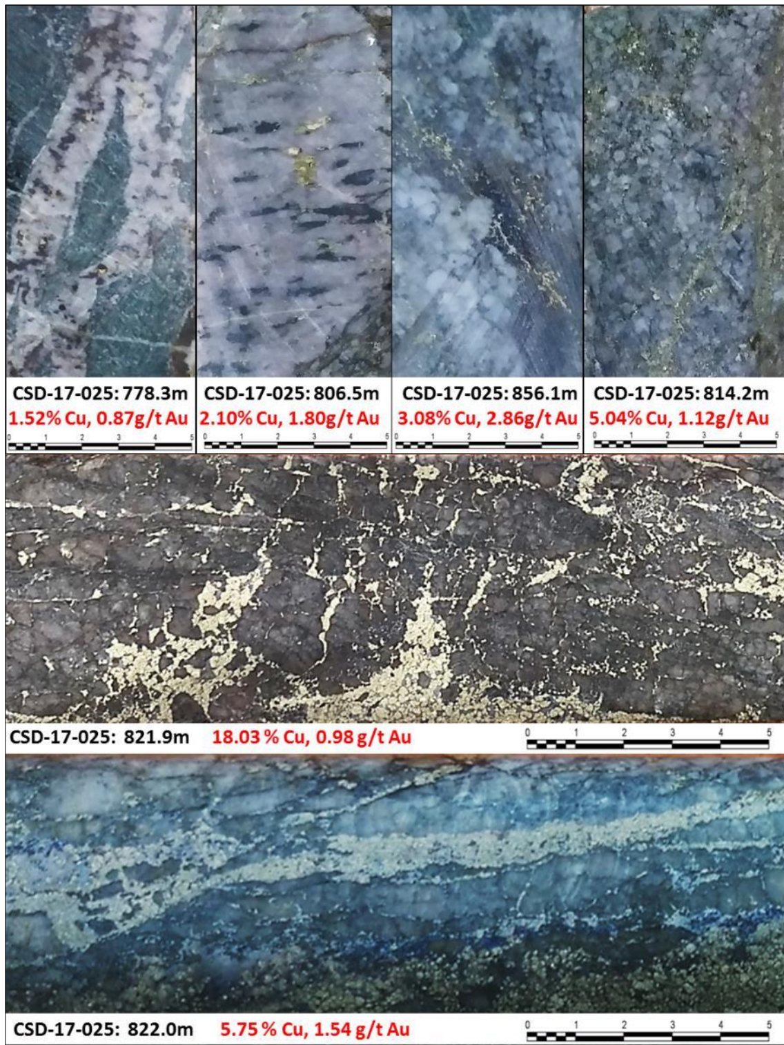
Figure 5: Selected examples of mineralisation encountered in Hole 25, showing the copper and gold assay results for two metre intervals that contain the drill-core images shown in the figure.
