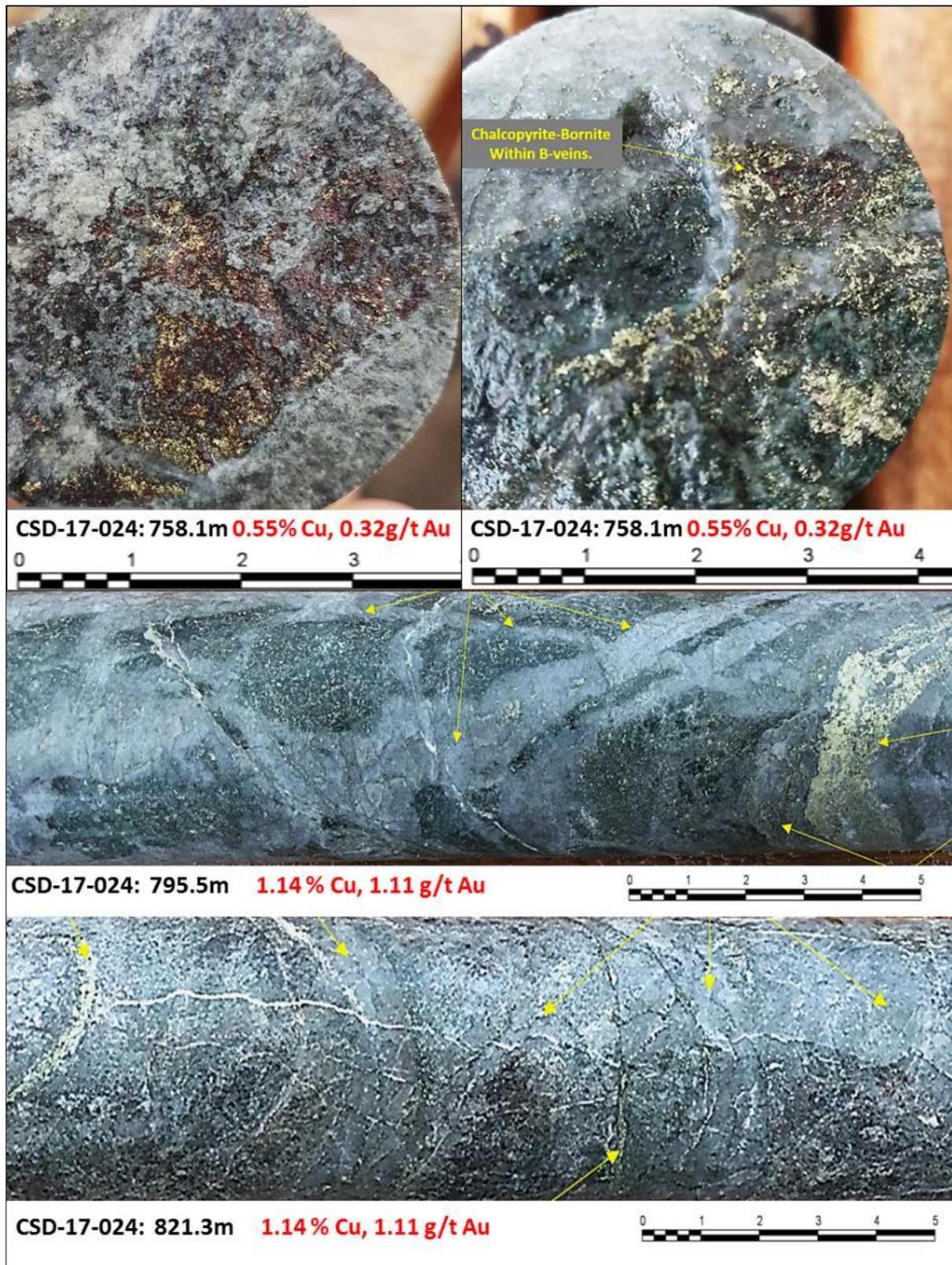
Figure 3: Selected examples of mineralisation encountered in Hole 24, showing the copper and gold assay results for two metre intervals that contain the drill-core images shown in the figure.
