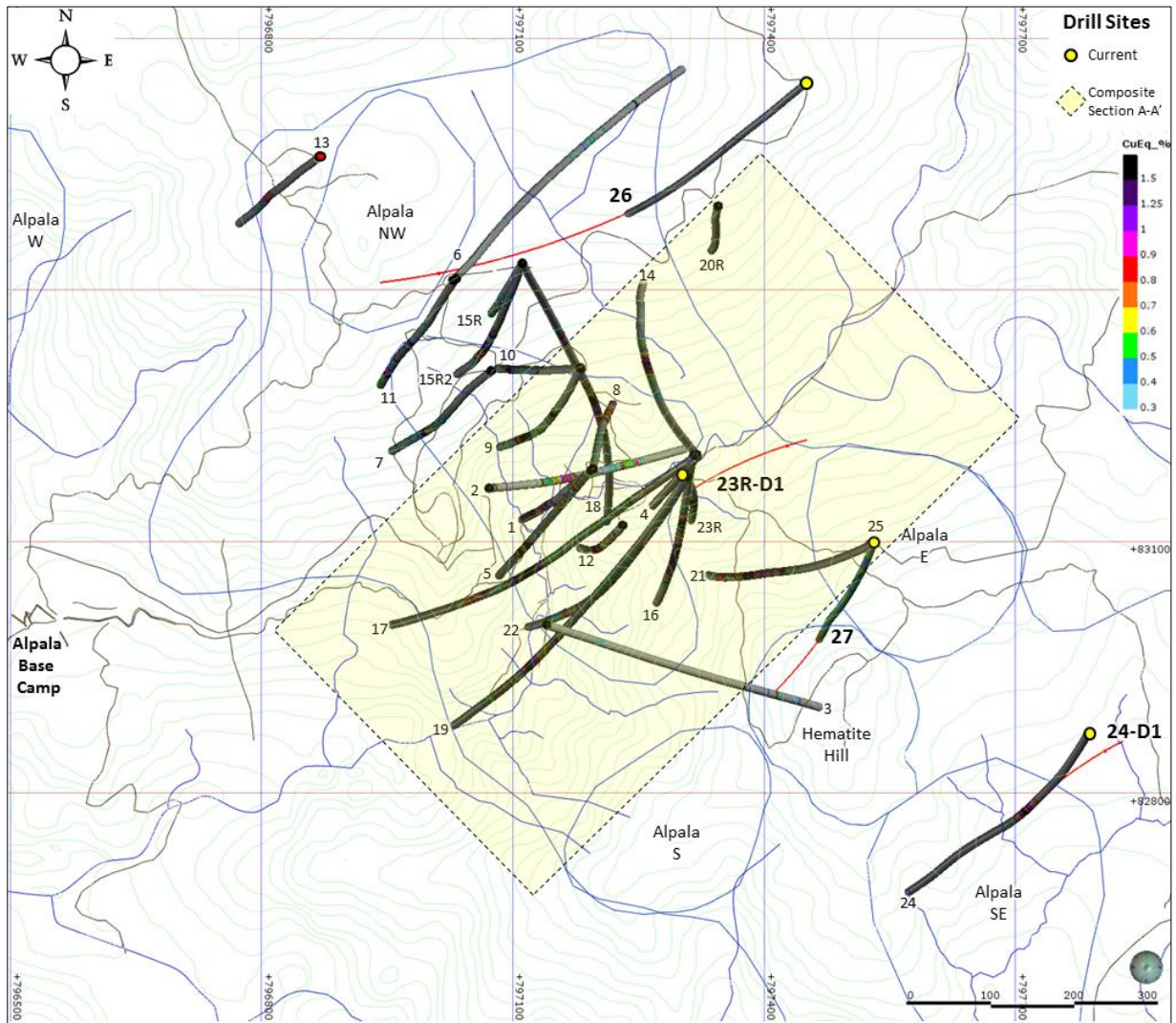
Figure 1: Drill hole location plan, showing existing drill holes and recently completed drill holes 23R, 24 and 25. The locations of active drill holes 23R-D1, 24-D1, 26 and 27 are also shown. Proposed drill hole locations, aimed at defining the geometry and extent of the greater Alpa porphyry copper-gold system, are shown in red. These holes include 23R-D1 and 24-D1. The northeast trending composite section (A-A') shown in Figure 4 is indicated by a yellow band with dashed lines.
