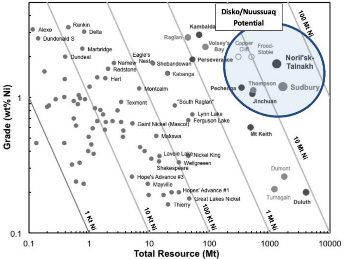
FIGURE 1: Diagram showing well known nickel-sulphide deposits/mining districts. The expected grade tonne range for Disko indicated inside the transparent blue ellipsoid, based on mass balance of depleted lavas. Source for the background data/original diagram: Leshner & Houli 2015: Magmatic Ni-Cu-PGE Mineralization in Canada. SGS Open House, Technical Session 3: Exploration Overviews and Tantato Domain Geoscience – Dec 2015. Ministry of Energy and Resources, Saskatchewan, Canada. ( https://publications.saskatchewan.ca/#/products/82536 )
