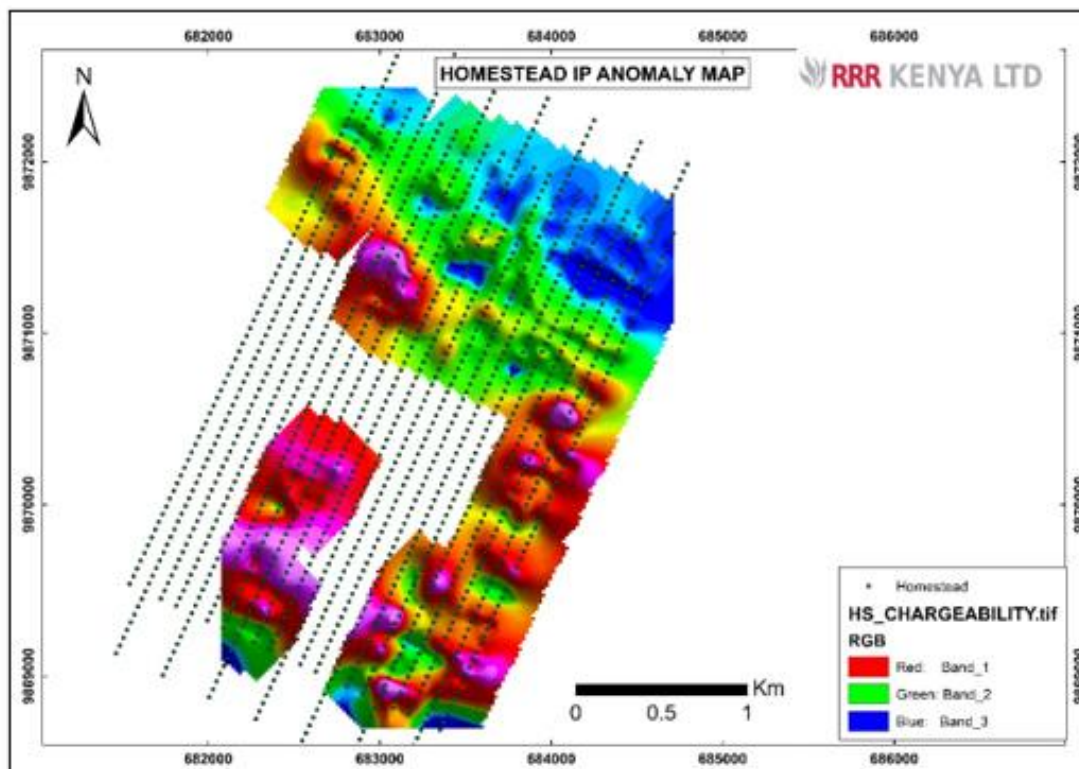
Homestead resistivity and chargeability maps of surveyed sections.
