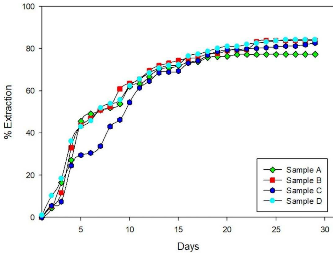
Figure 2: % Extraction of gold for the various days
