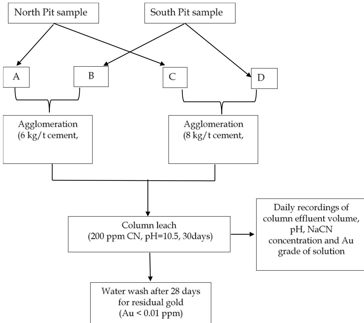
Figure 1: Flowsheet for Column Leach Test Work
