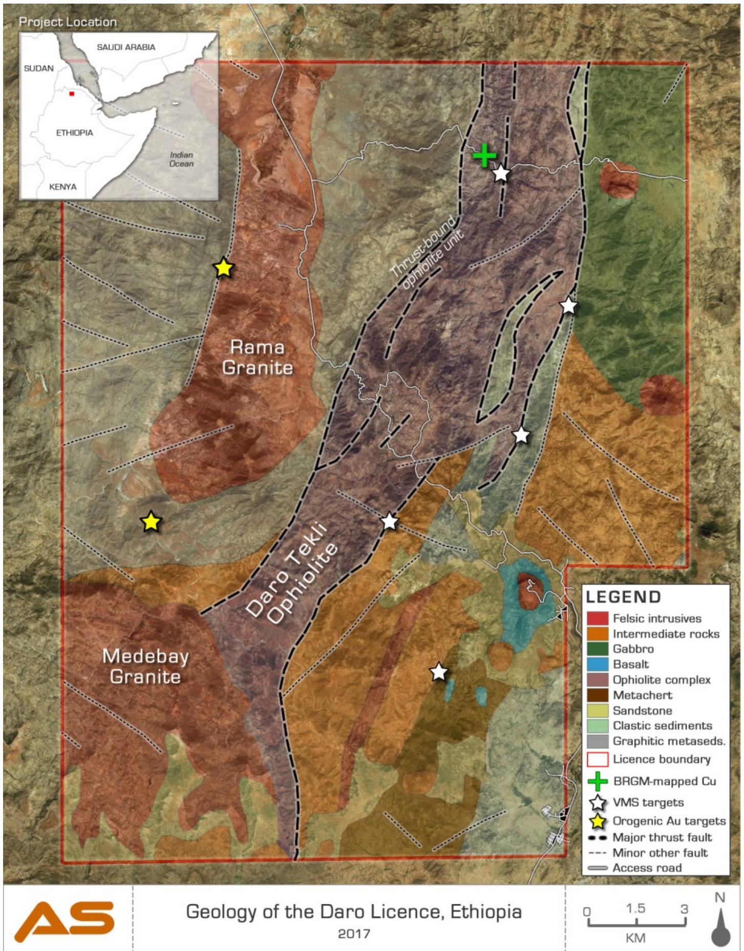
Figure 2: Geology and structures of the Daro licence
