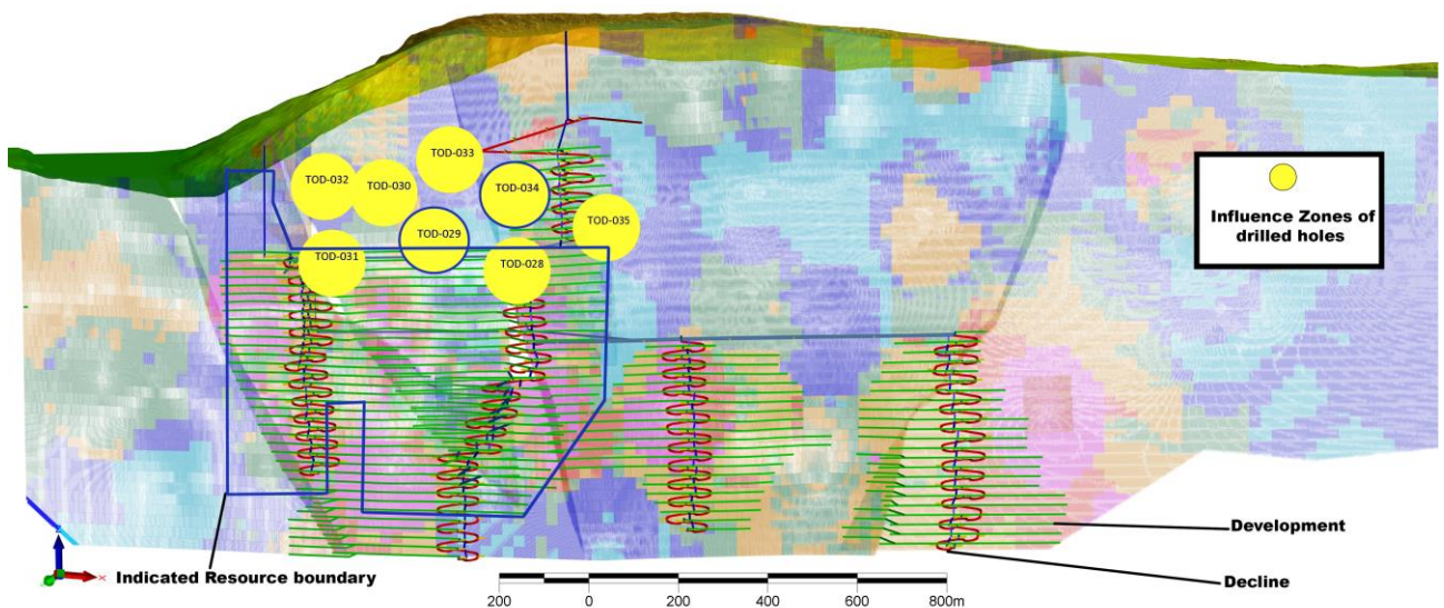
Figures 2 & 3: East-West long sections locating completed primary drill holes with assays for holes TOD-032, TOD-033, TOD-034 and TOD-035 and all additional holes completed during the 2021 drill campaign (Yellow).
