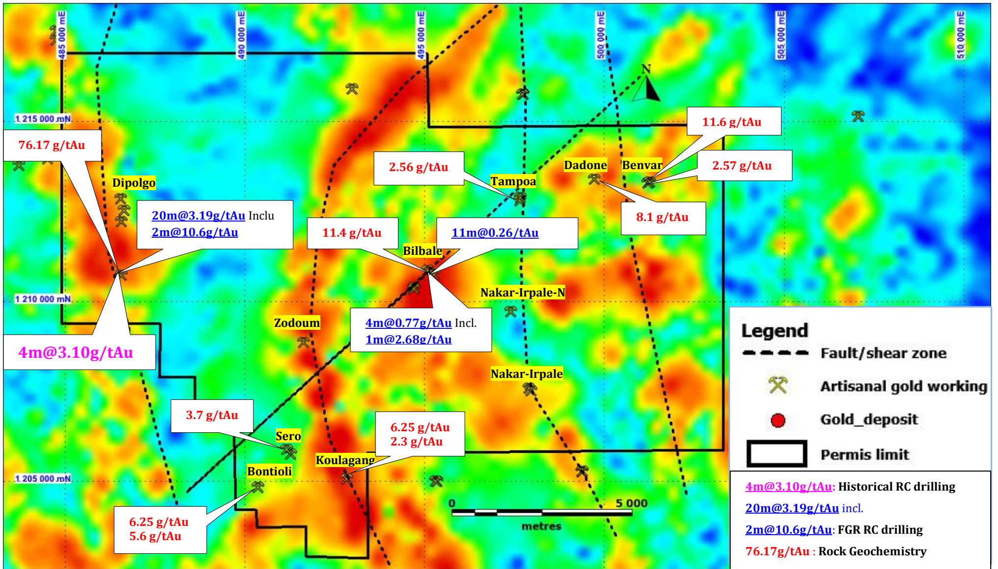
Fig1.: Bilbale rock geochemistry, RC drilling results and artisanal gold working sites in the Bilbale licence
