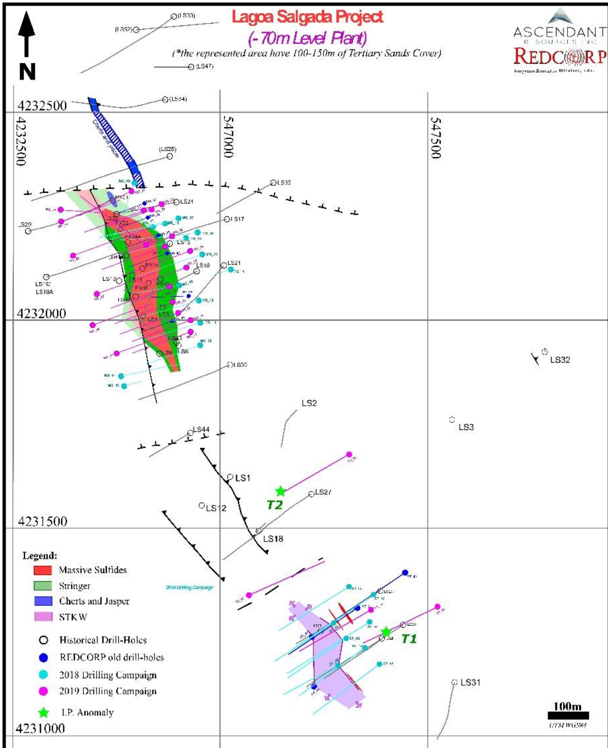
Figure 2: Plan View of the All Drill Holes for Lagoa Salgada
