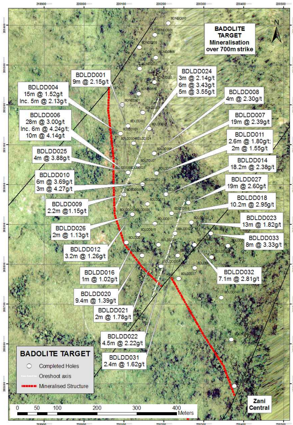
Figure 2: Drill results at end March 2011 with an average cut off grade of 1g/t, Badolite area. All holes vertical.
