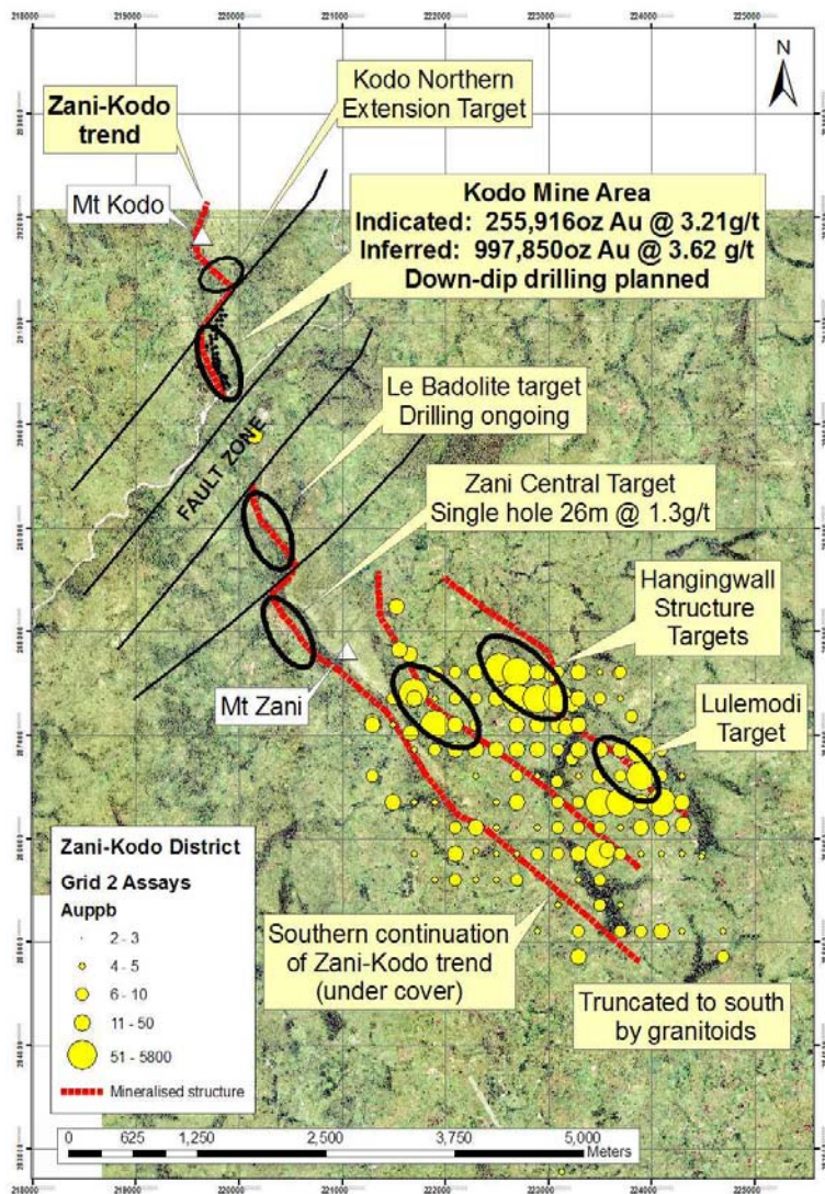
Figure 1: Zani-Kodo trend showing the position of Badolite target area, Zani-Kodo project.
