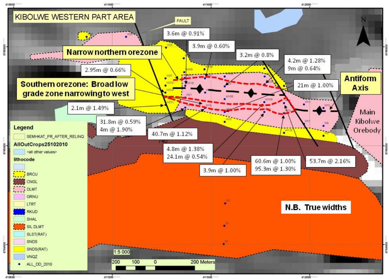
Figure 3: Position of all results, Kibolwe West project.
