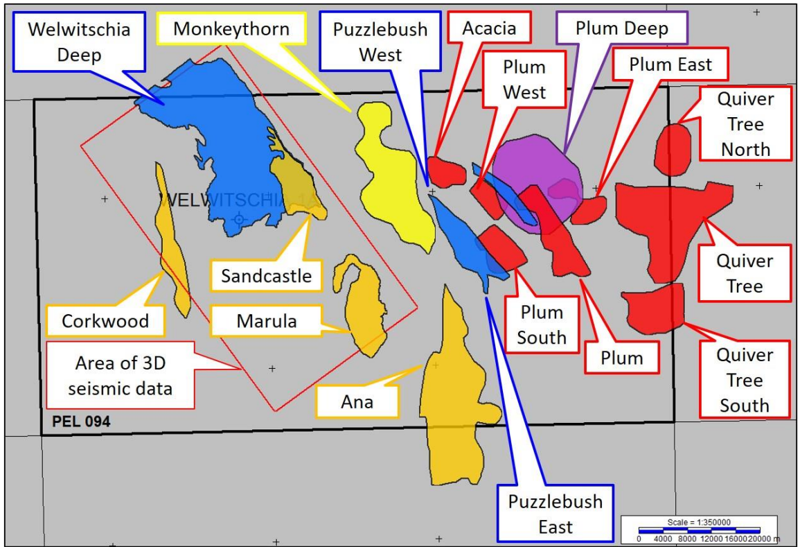
Figure 2: Prospect and lead portfolio map for Global's Namibian licence PEL0094. The features not listed in Table A are lead areas, which require more work to be considered leads or prospects
