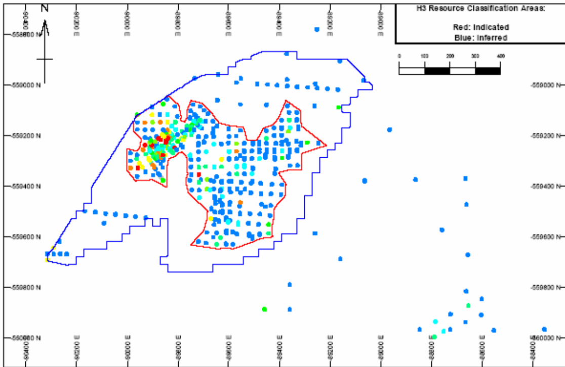
Figure 3.13 H3 Detail - Borehole Location Plan and Resource Classification Areas
