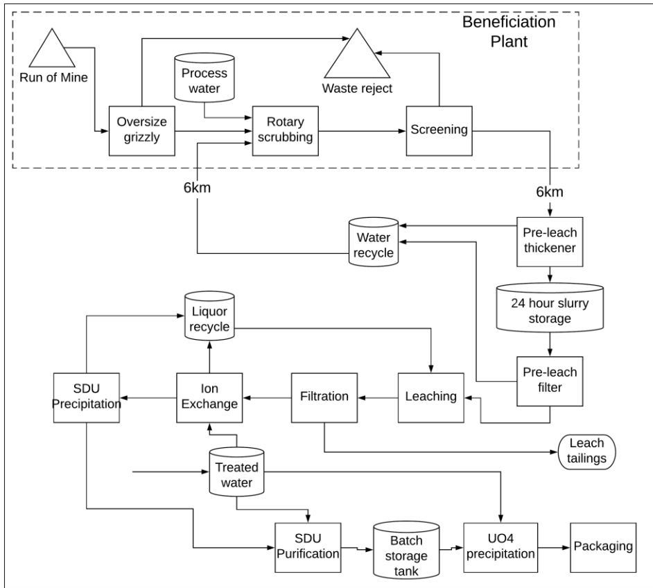
Figure 5. Tiris Uranium Project Process Block Flow Diagram
