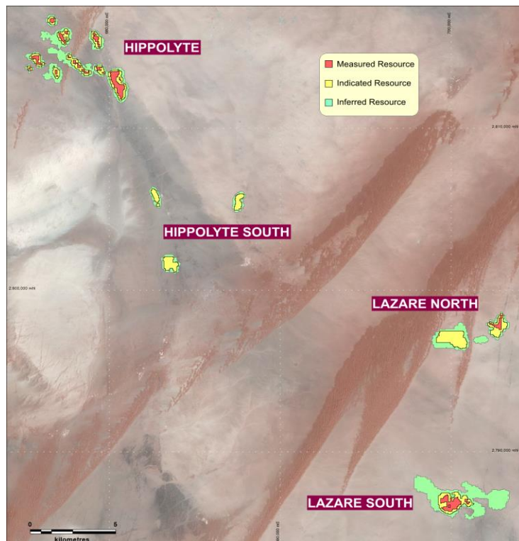
Figure 4. Location of 2018 Tiris Resource Estimate Zones
