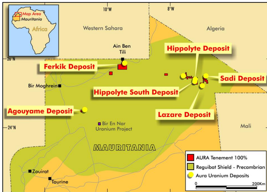
Figure 3. Location of Aura's Tiris Uranium Resources
