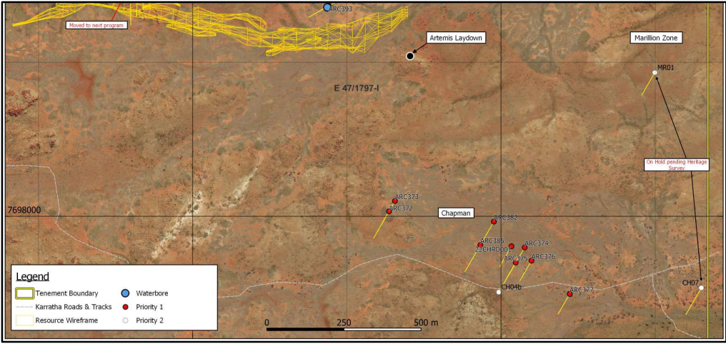
Figure 7: Chapman location map with drill collars (red).
