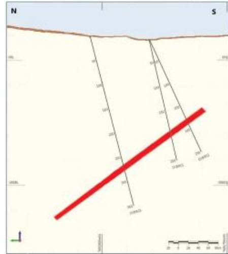
Figure 2: Modelled Osborne conductor
