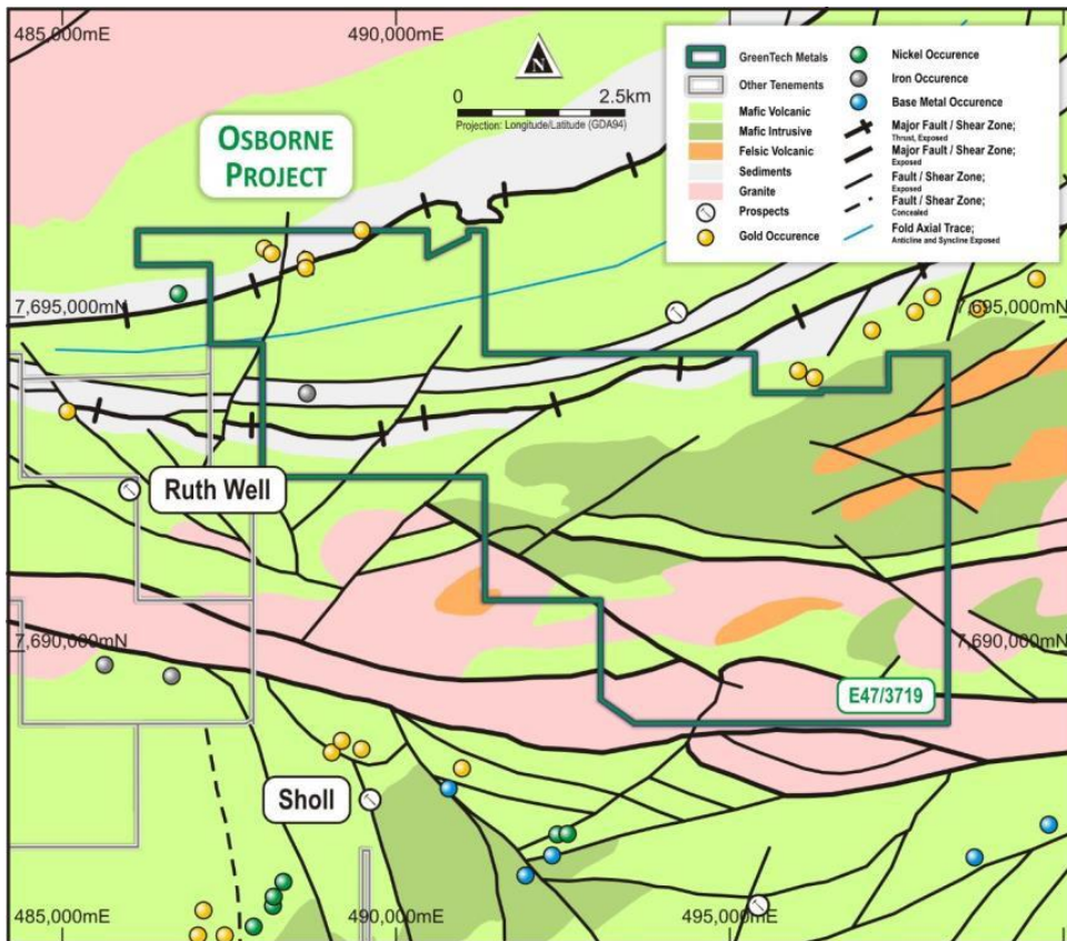
Figure 3: Local geology of the Osborne Nickel prospect (Source GSWA 1:500,000 Digital geological map with units modified to simplify legend. MGA94 Zone 50 coordinates)
