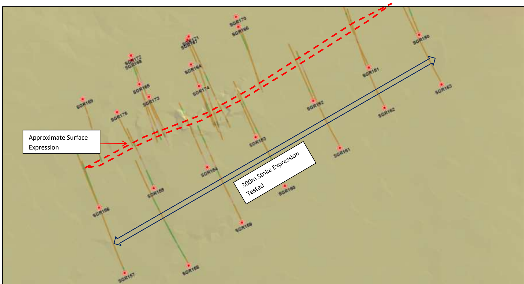
Figure 2: Lidar DTM (Transparent) – Drill traces & Schematic Surface Expression of Mineralised Zone Superimposed
