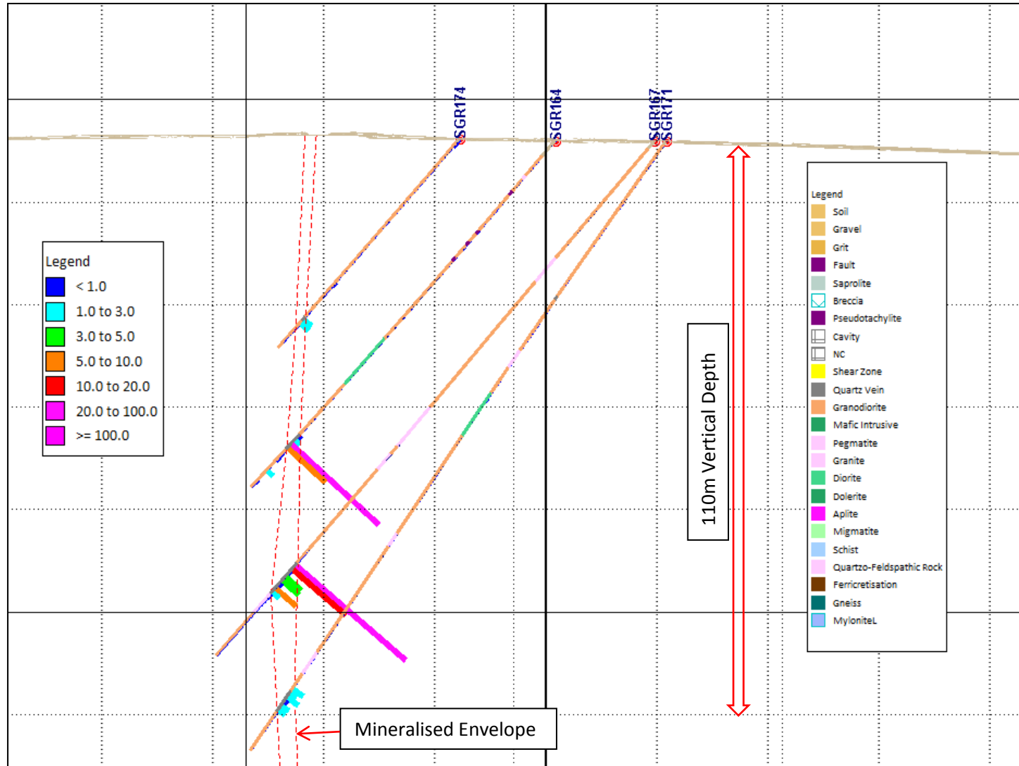
Figure 3: Section - Drill Traces, Geology, Grade and Envelope of Mineralised Zone
