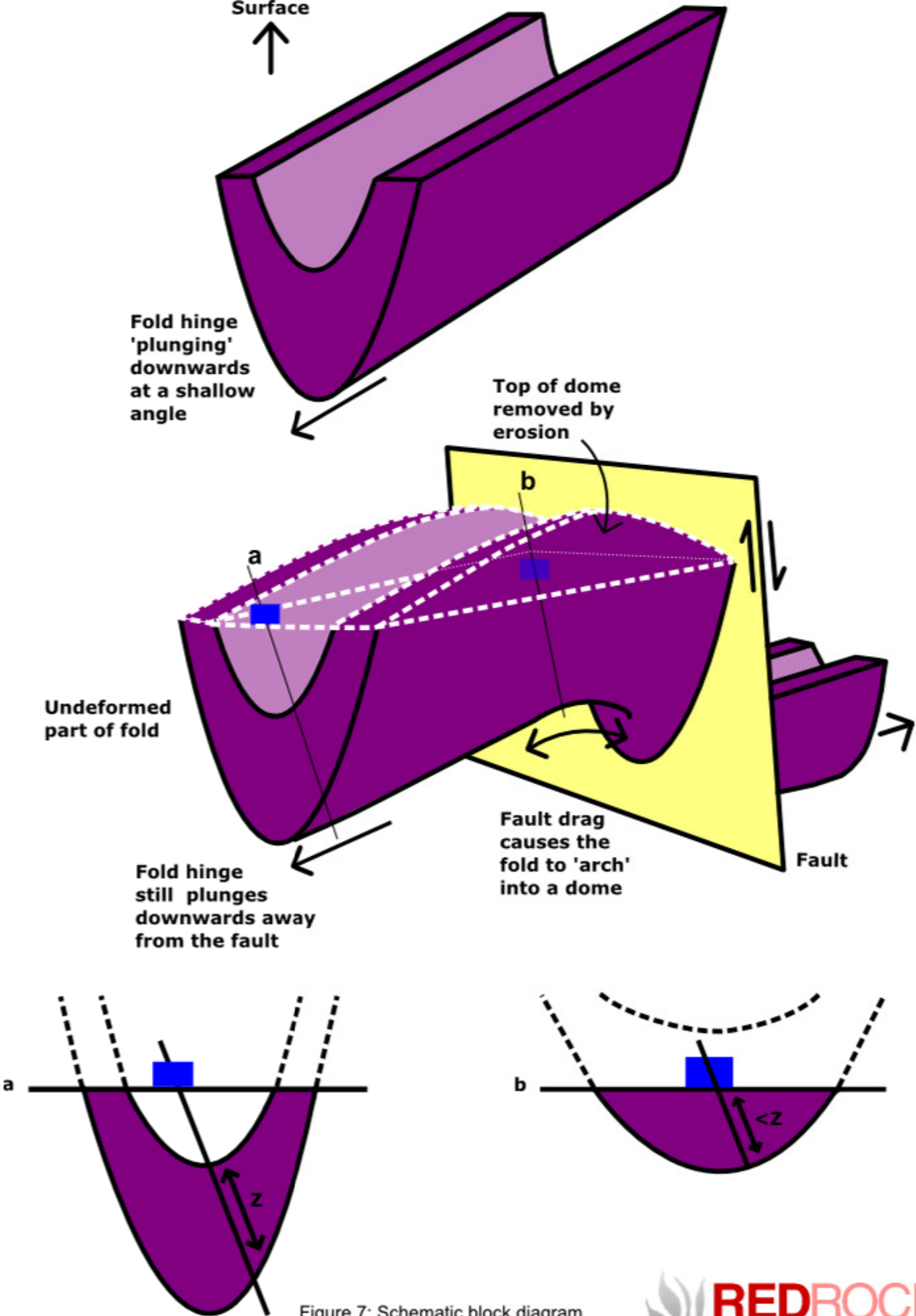
Figure 7: Schematic block diagram demonstrating fold geometry at Havik Northeast
