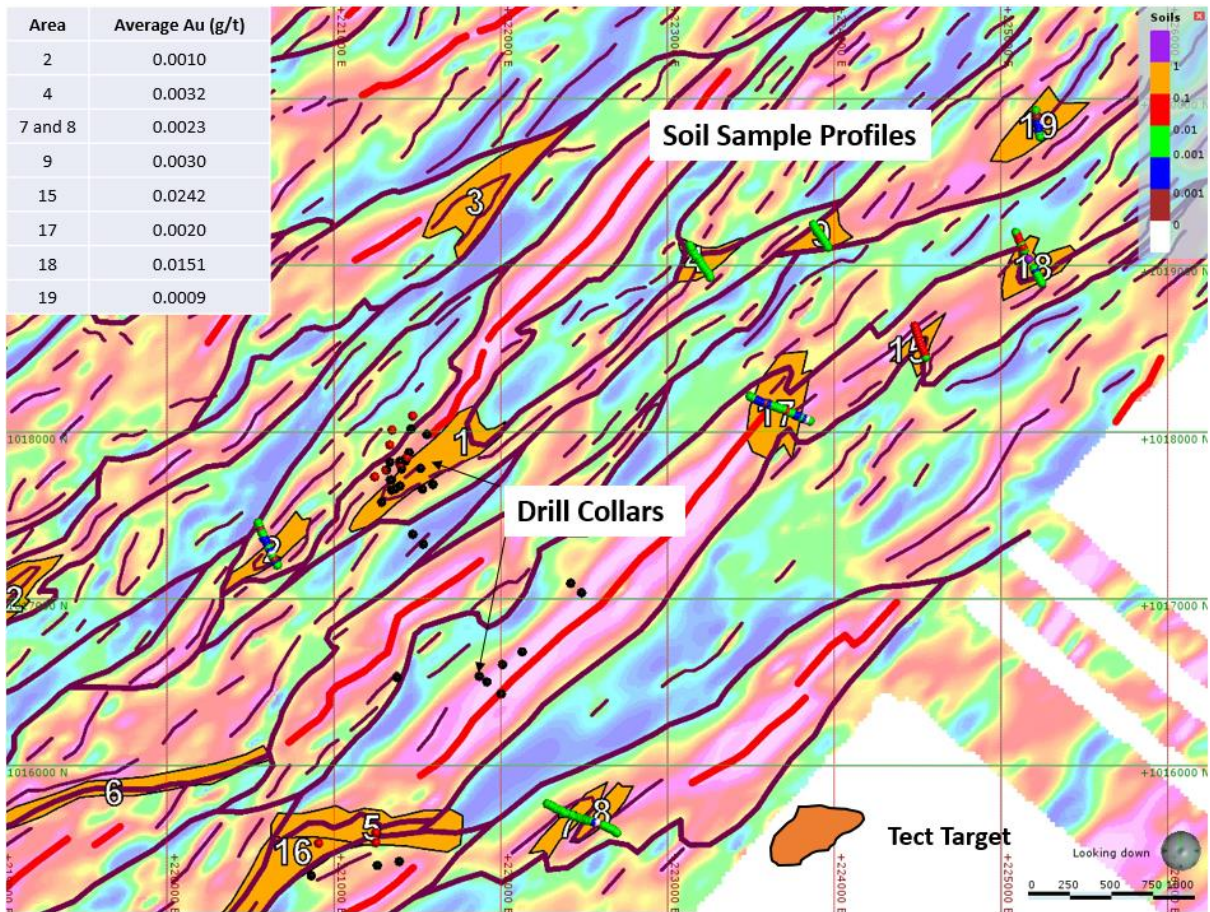
Figure 2: Summary of soil sampling results against the identified structural targets (0.0001 g/t Au detection limit)
