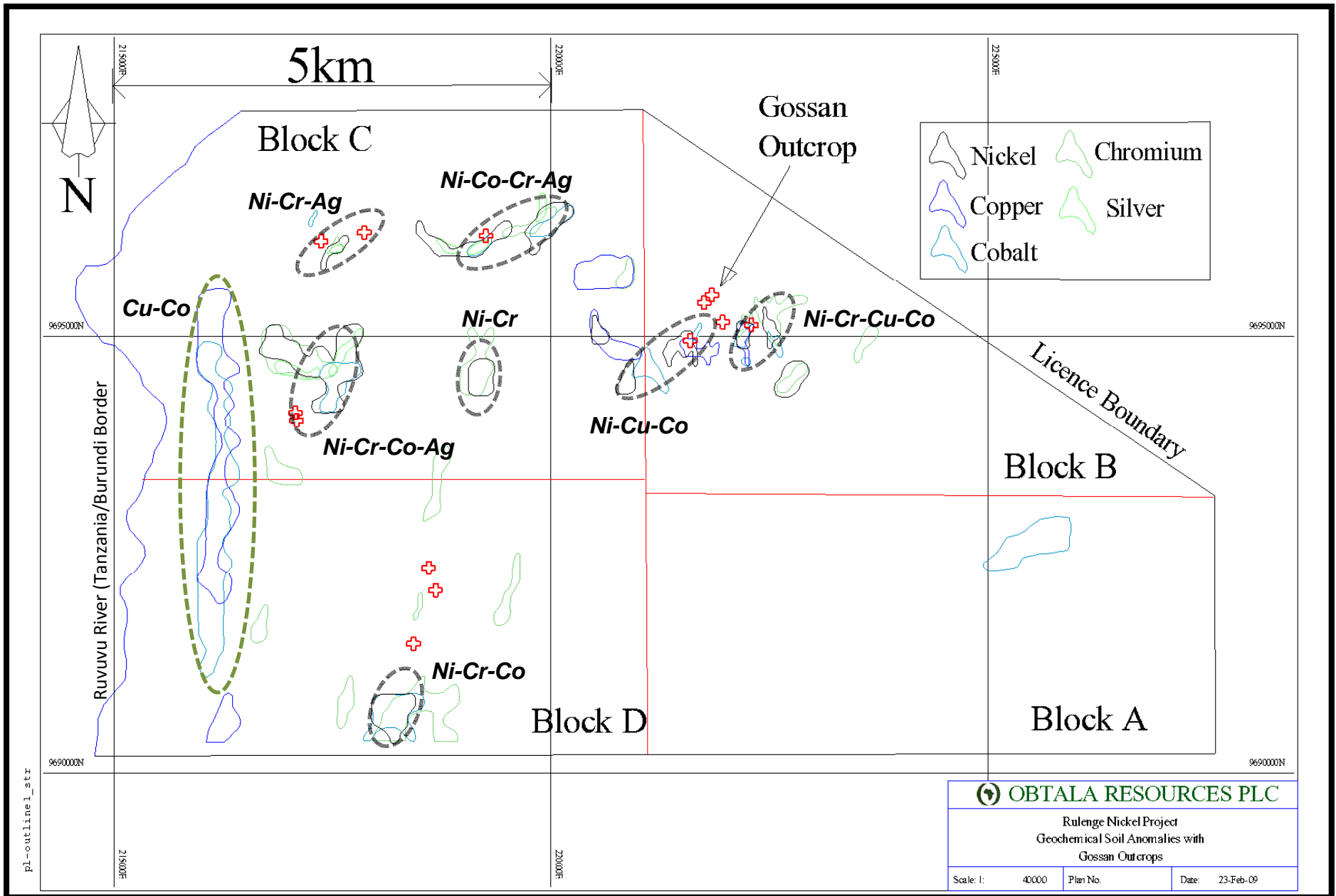
Rulenge Nickel Project : Soil Geochemical Anomalies (February 2009)
