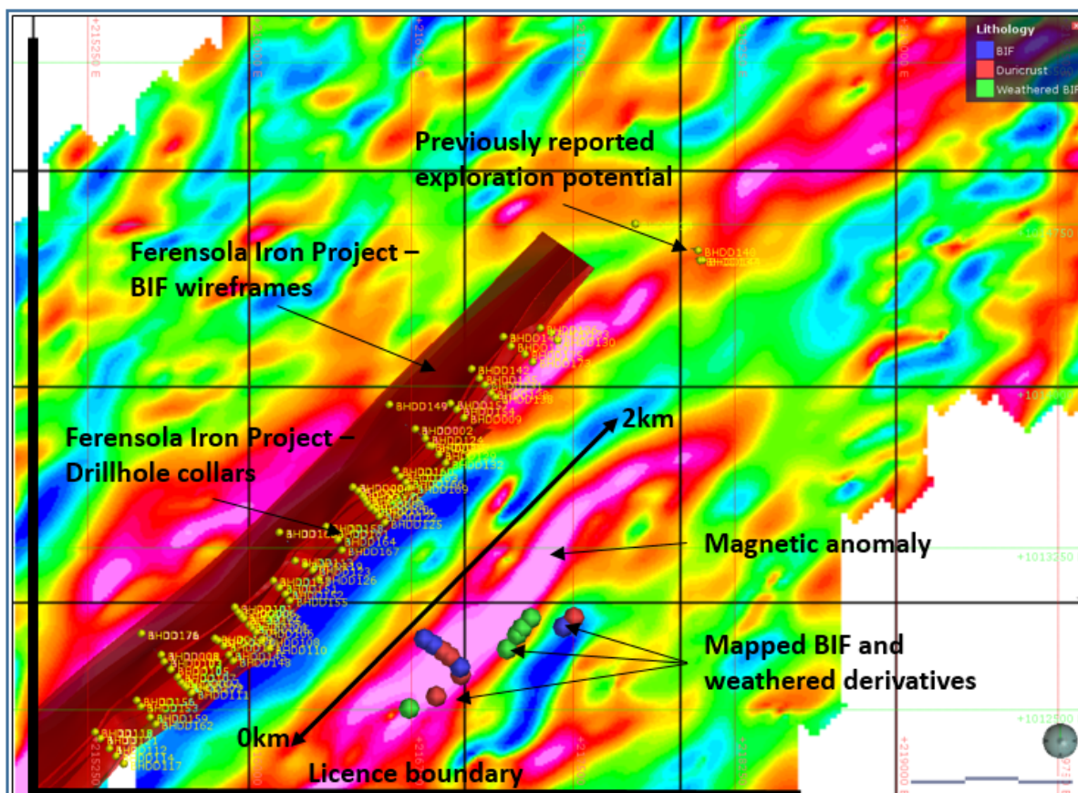
Figure 1: Location of mapped Banded Iron Formation and weathered derivatives lying to the southeast of the Ferensola Iron project
