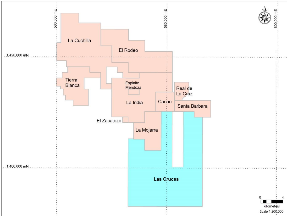
Figure 1 Location of the Las Cruces concession within the La India Project area.
