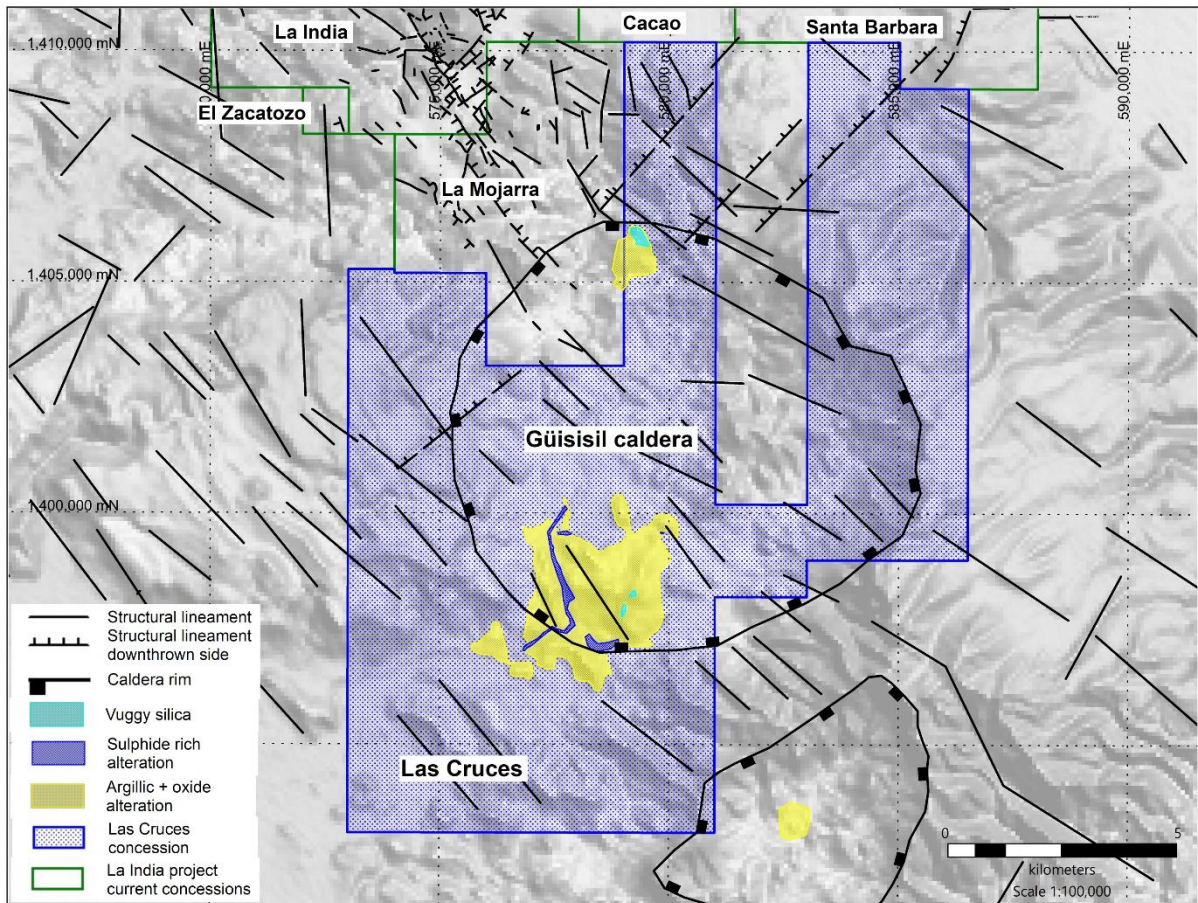
Figure 2 Location of the Güisisil caldera and alteration zones within the Las Cruces concession.
