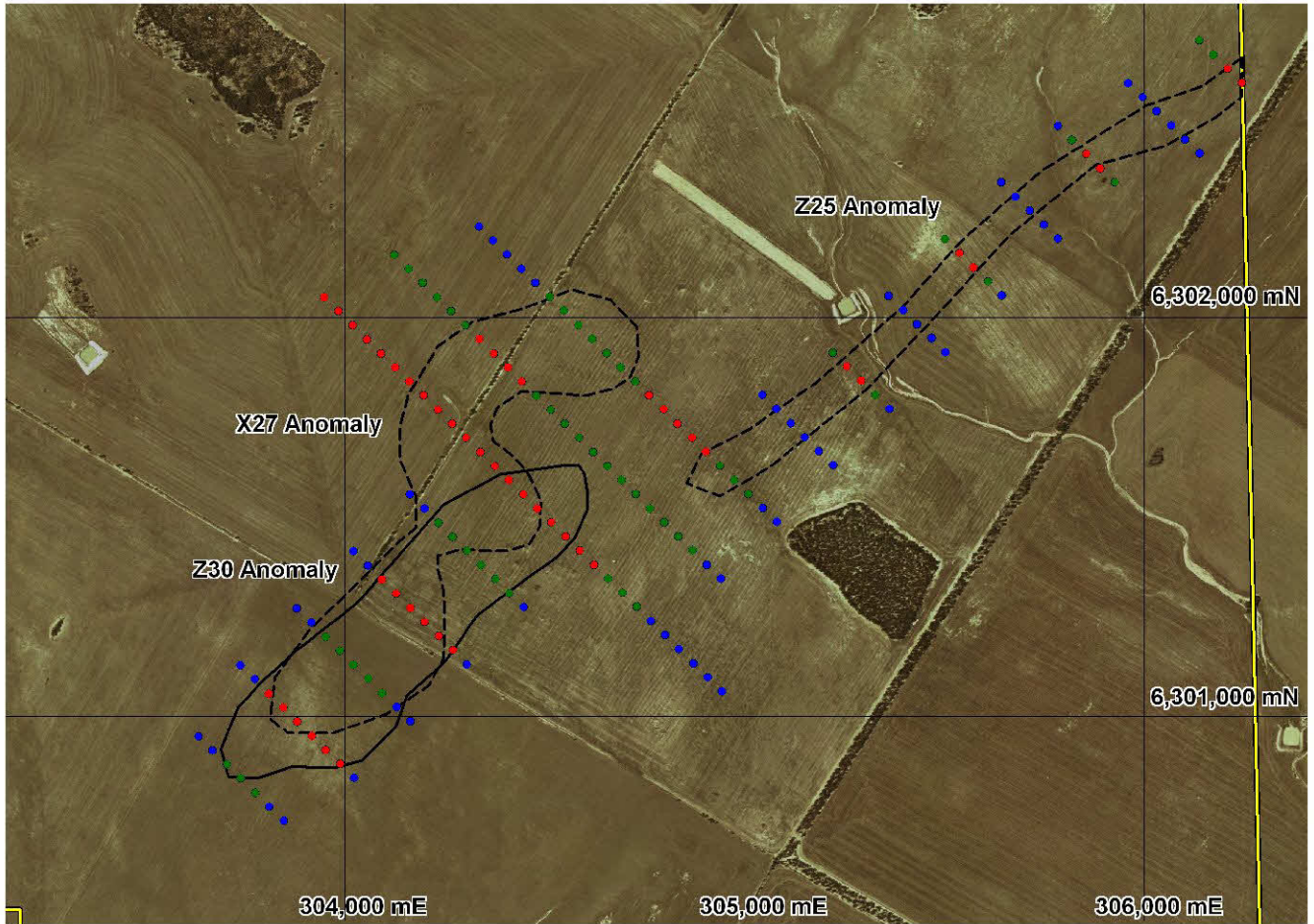
Figure 27: T1: Combination of AEM anomalies to be drill tested along NE trending structure.
