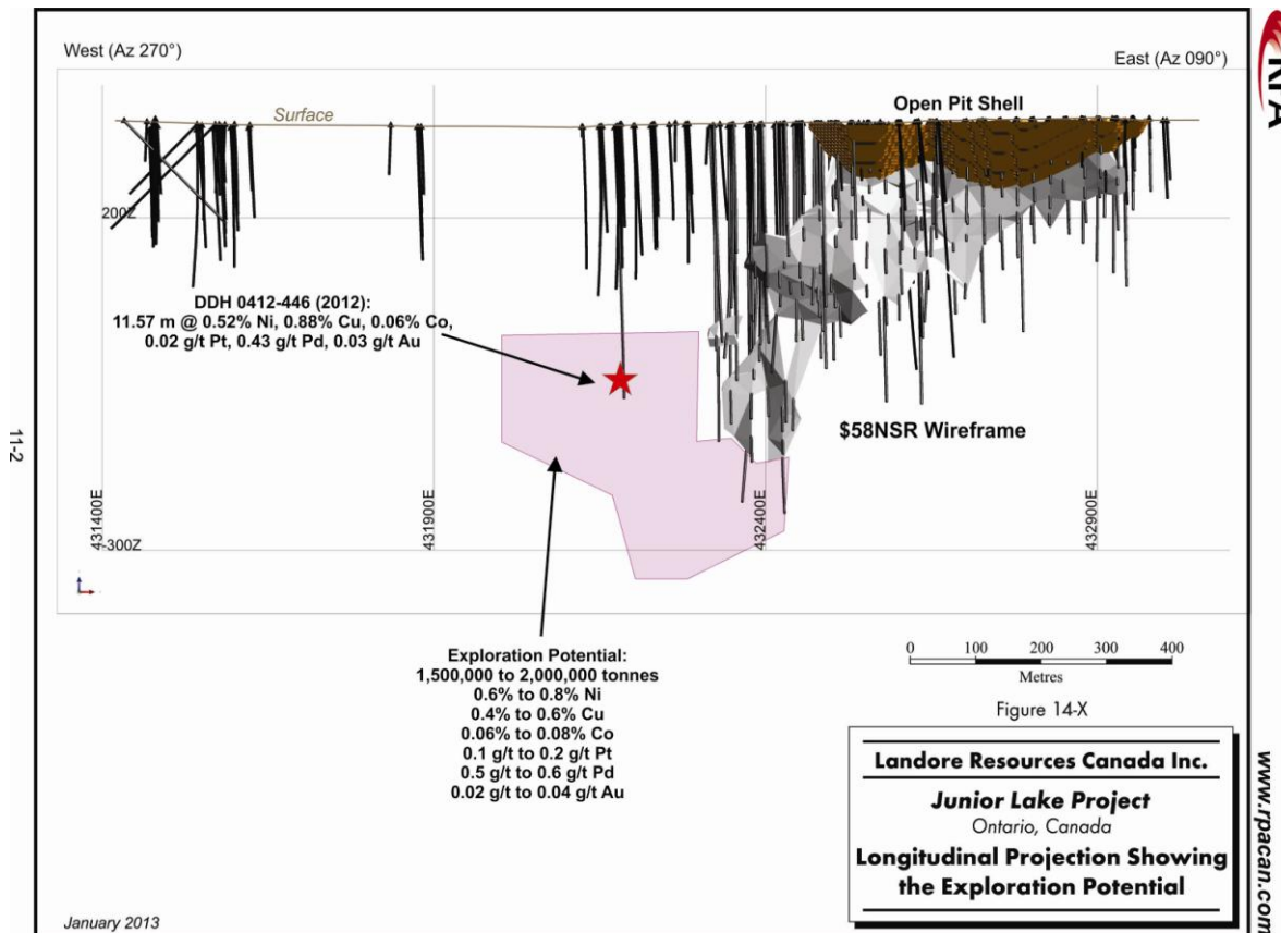
FIGURE 2 LONGITUDINAL PROJECTION OF THE EXPLORATION POTENTIAL
