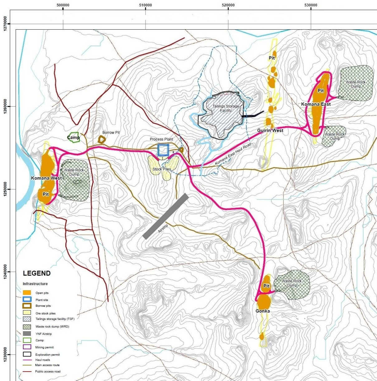
Figure 2: Gonka Deposit
