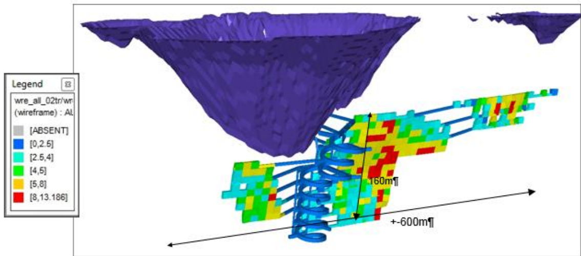
Figure 1: Gonka open pit and underground mine plan
