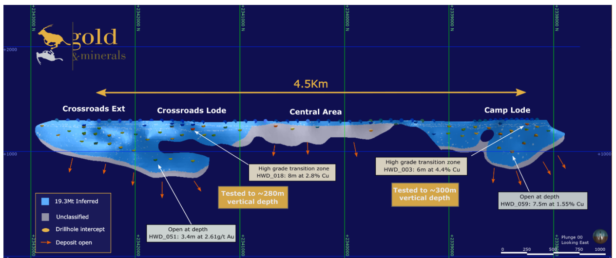
Hawiah Long Section showing Key Drilling Results and Lodes
