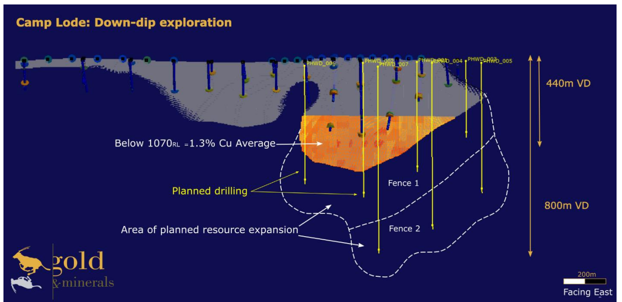
Long Section showing Planned Drilling and Resource Potential below current Camp Lode Mineral Resource
