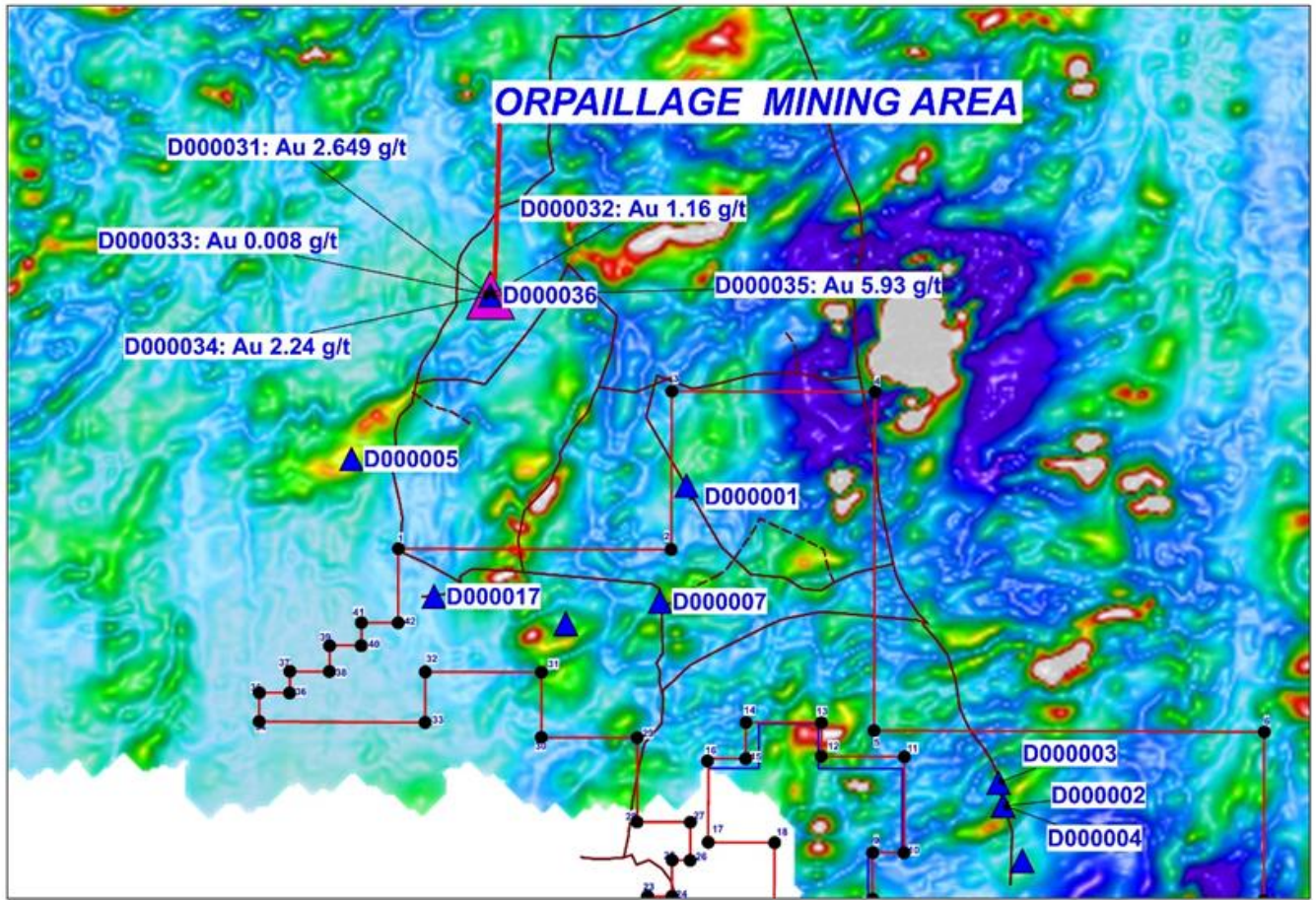
Fig 3: Djekanou license: rock chip samples
