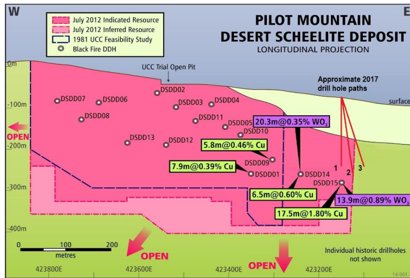
Figure 2: Desert Scheelite drill intersections viewed in long section looking northwards. Proposed drill targets and hole paths shown at the eastern (right hand) end.
