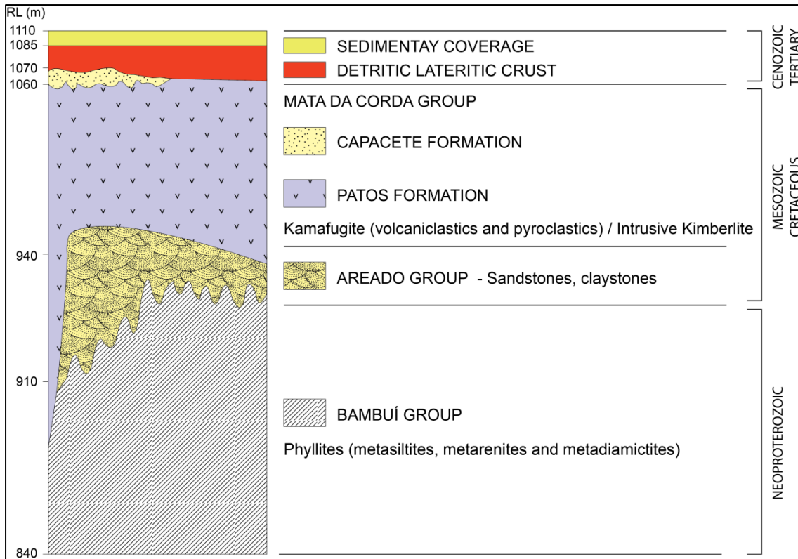
Figure 8 – Stratigraphic column for Maximus Prospect area.
