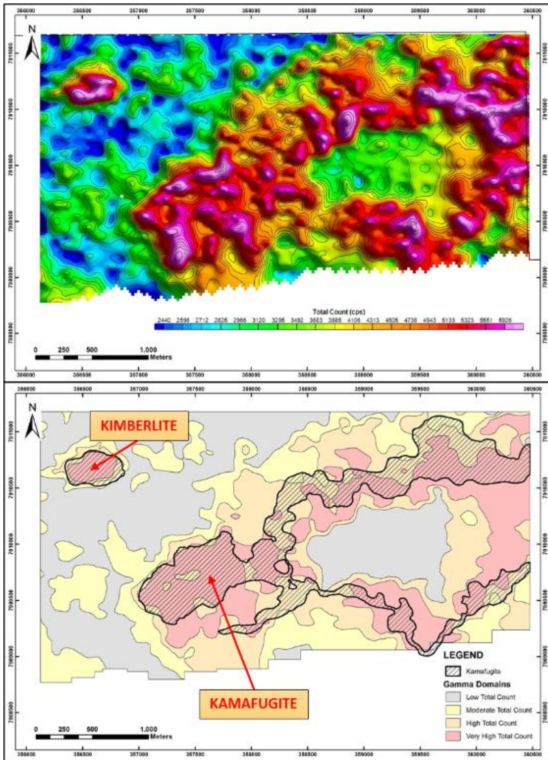
Figure 4 – Total Count map and the gamma-spectrometric domains.
