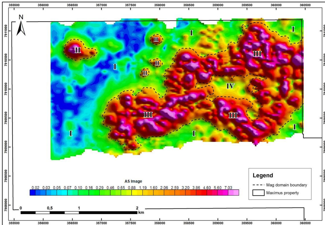
Figure 2 – Analytical Signal Image with the different magnetic domains identified.
