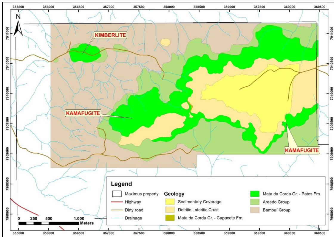
Figure 1 – Maximus Prospect Geological Map.
